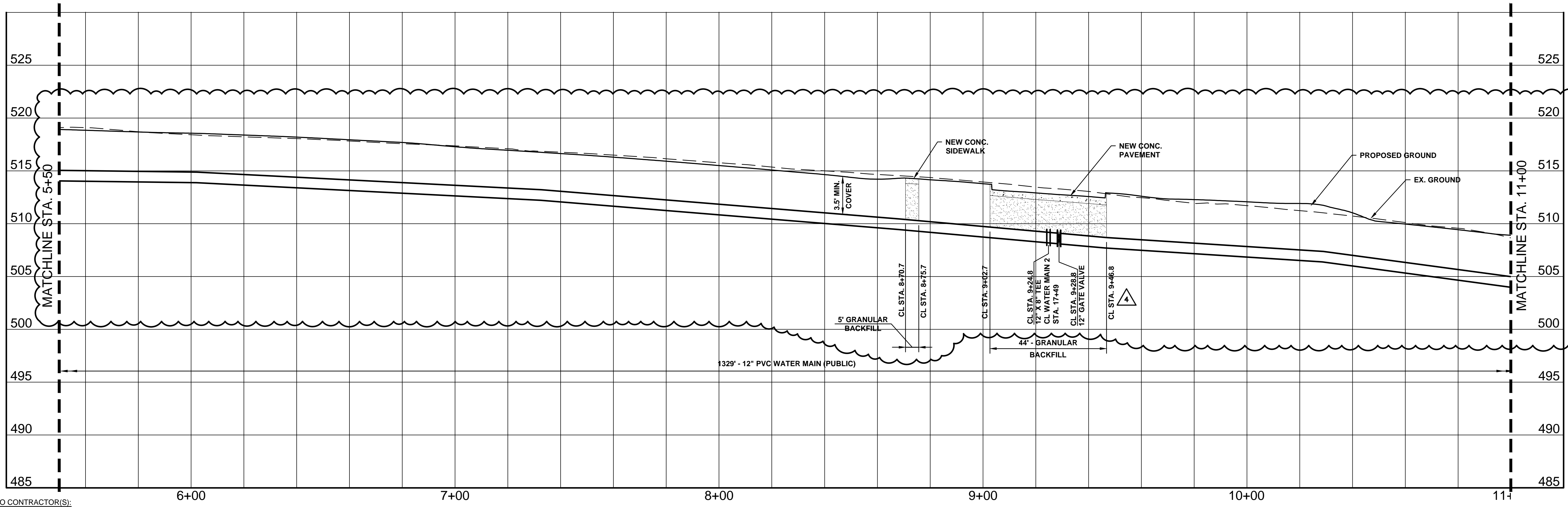
WATER MAIN 1 PROFILE SCALES: 1" = 20' HORIZONTAL 1" = 5' VERTICAL
