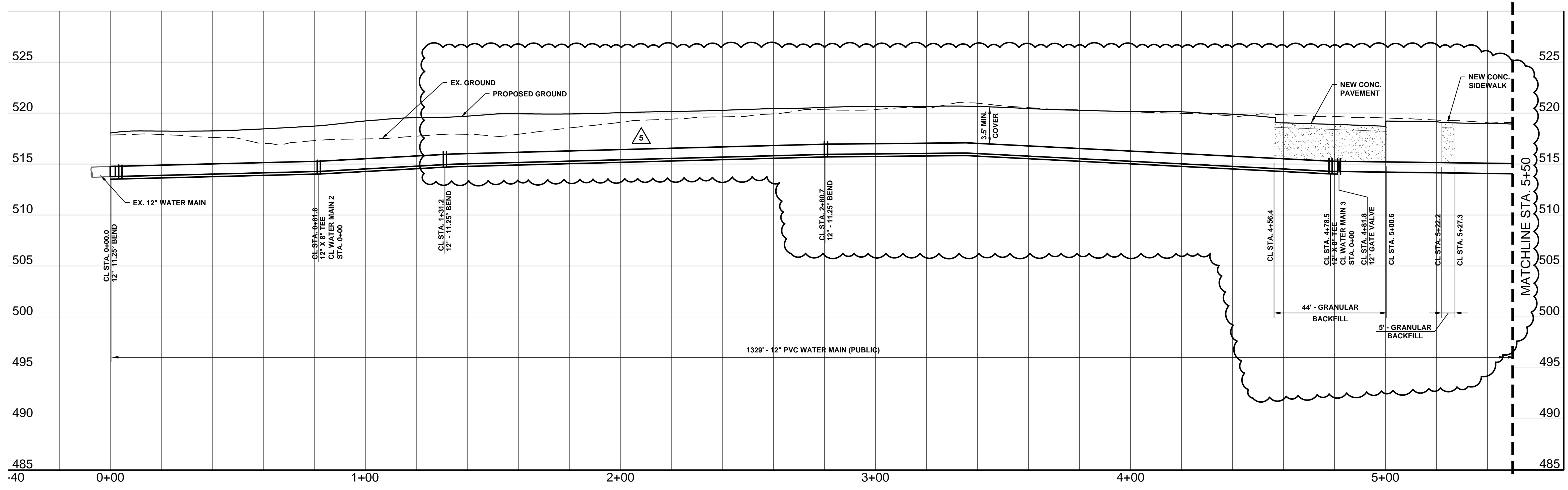
WATER MAIN 1 PROFILE SCALES: 1" = 20' HORIZONTAL 1" = 5' VERTICAL
