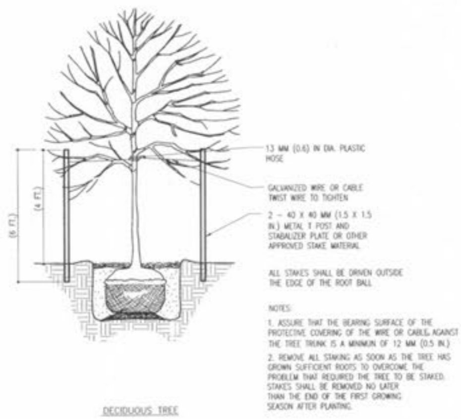
C3 TREE STAKING DETAIL L201 NIS
