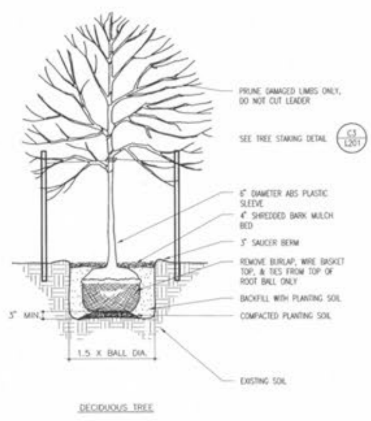
C1 TREE PLANTING DETAIL L201 NIS
