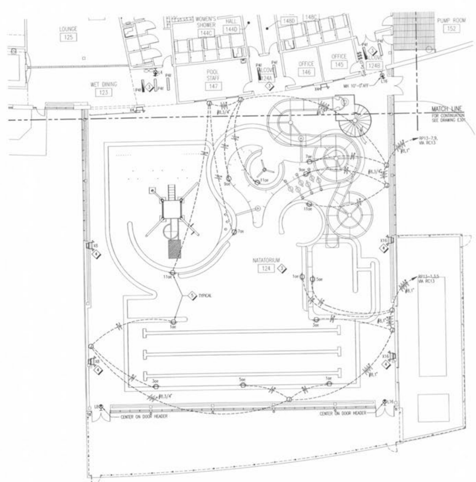
A1 FIRST FLOOR SOUTH LIGHTING PLAN E302 1/8" = 1'-0"
