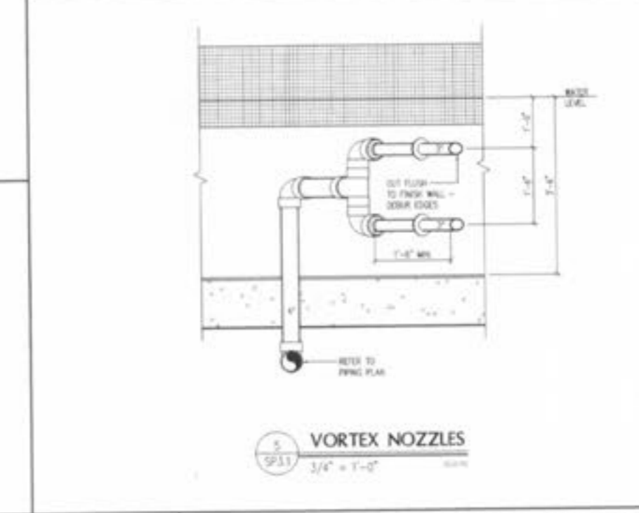
4 CONCRETE MAIN DRAIN 3/4" = 1'-0"
