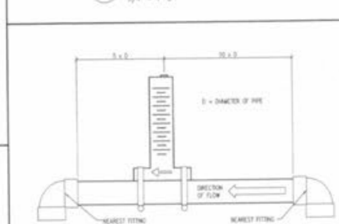
7 IMPACT FLOW METER 3/4" = 1'-0"
