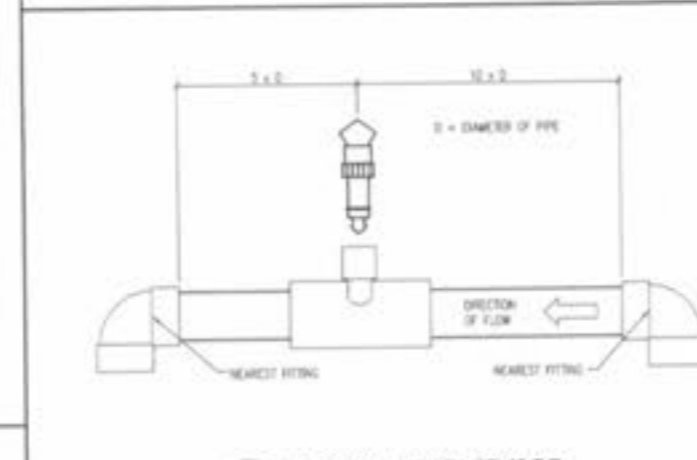
8 FLOW METER SENSOR 3/4" = 1'-0"
