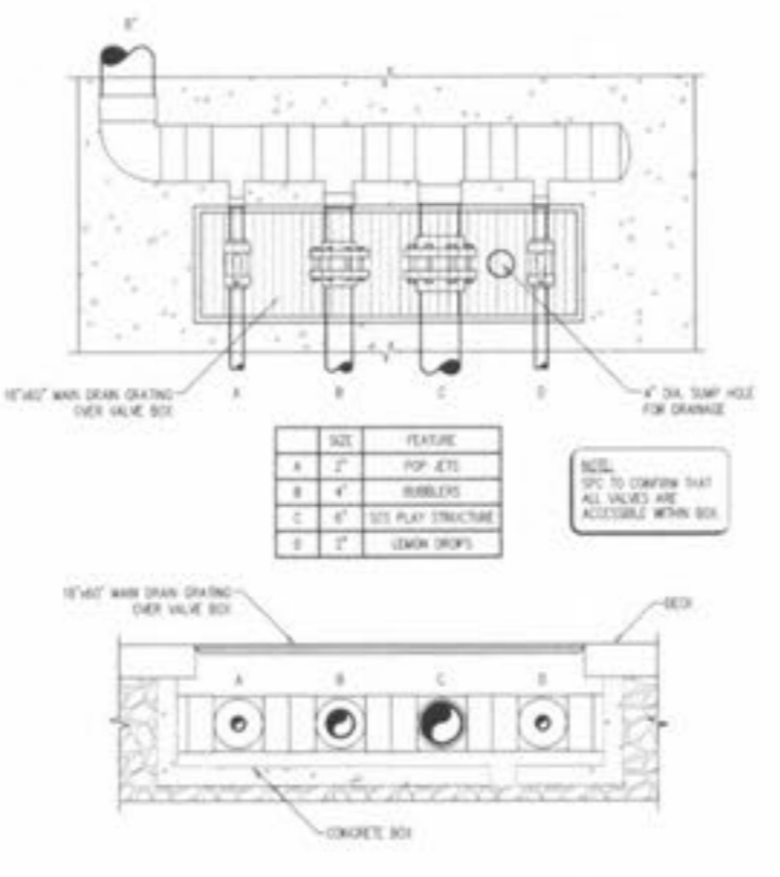
6 PLAY FEATURE VALVE BOX #1 3/4" = 1'-0"
