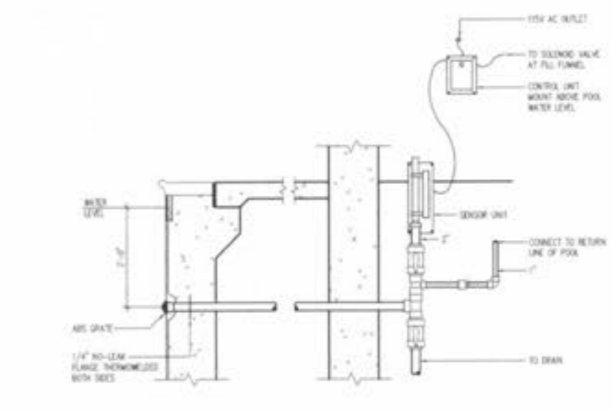
2 WATER LEVEL CONTROLLER 3/4" = 1'-0"
