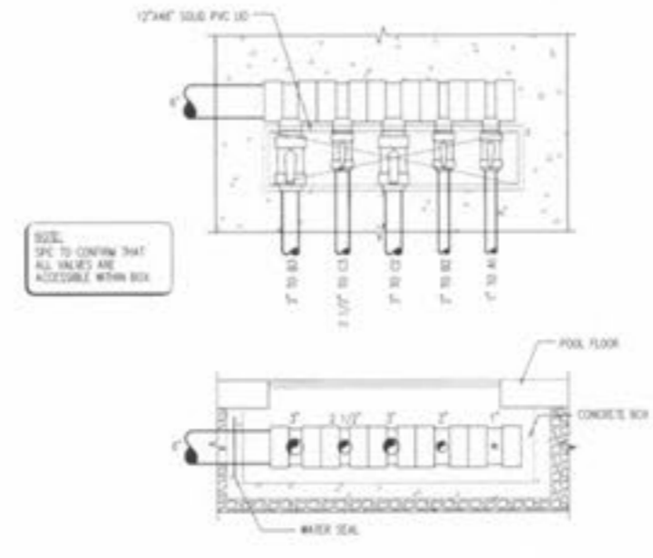
5 SCS 110 VALVE BOX 3/4" = 1'-0"
