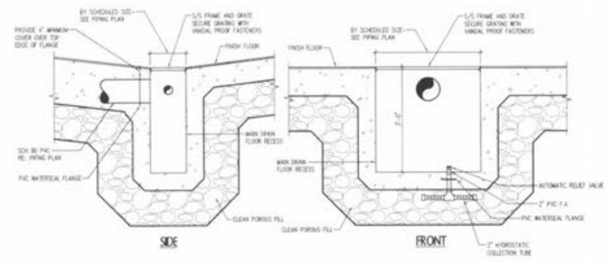
3 DEEP MAIN DRAIN 3/4" = 1'-0"
