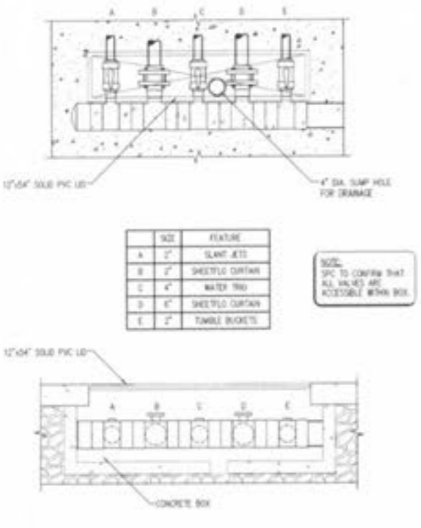
7 PLAY FEATURE VALVE BOX #2 3/4" = 1'-0"
