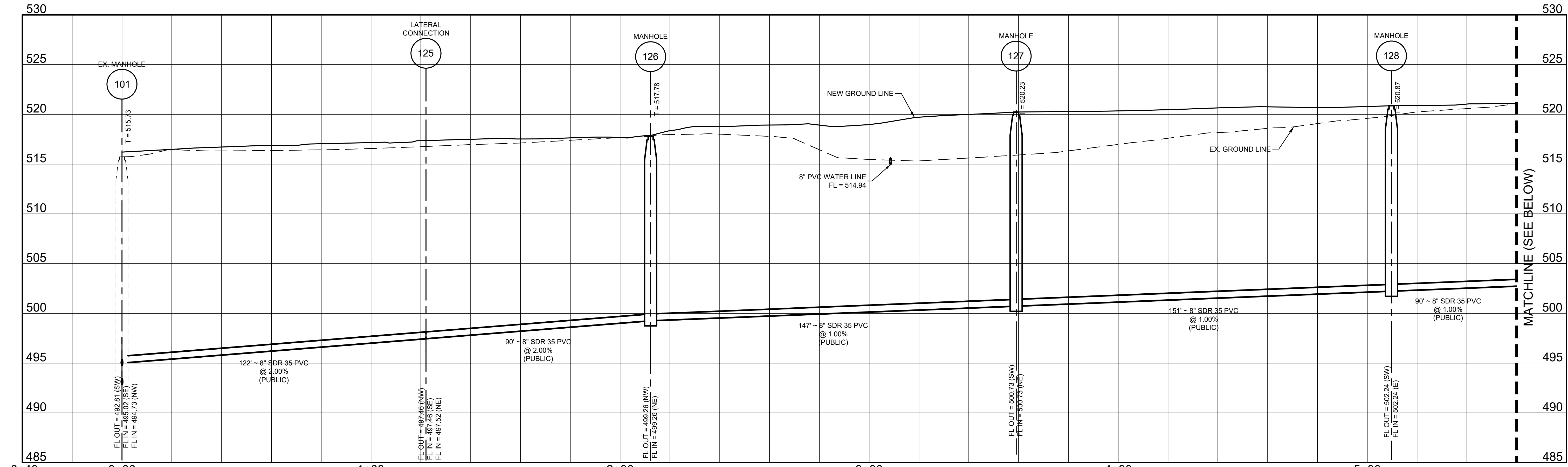
SANITARY SEWER PROFILE SCALES: 1" = 20' HORIZONTAL 1" = 5' VERTICAL
