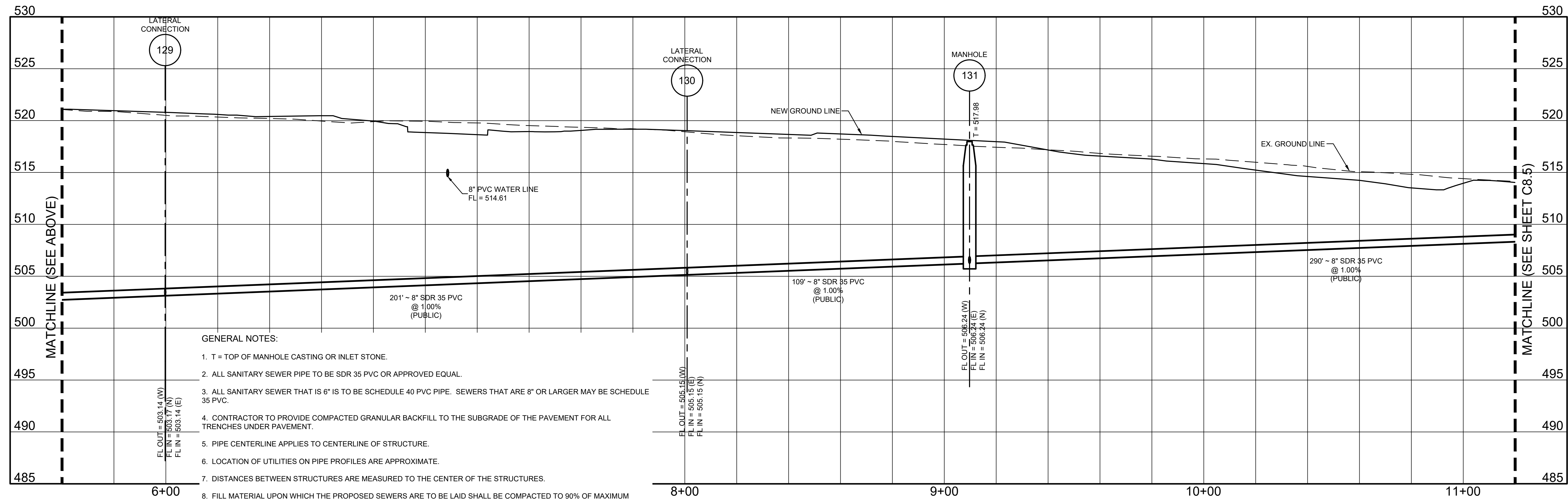
SANITARY SEWER PROFILE SCALES: 1" = 20' HORIZONTAL 1" = 5' VERTICAL
