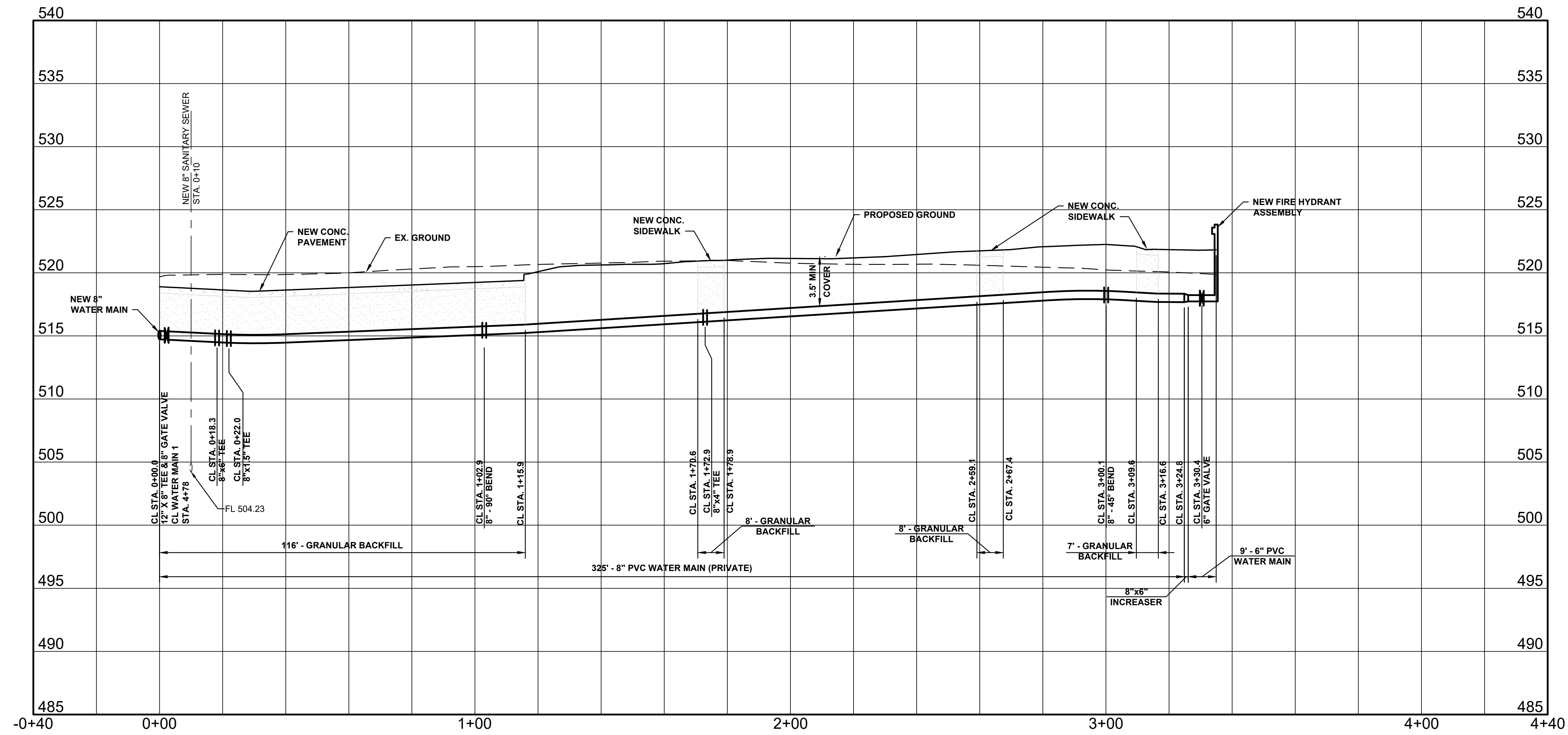
WATER MAIN 3 PROFILE SCALES: 1" = 20' HORIZONTAL 1" = 5' VERTICAL
