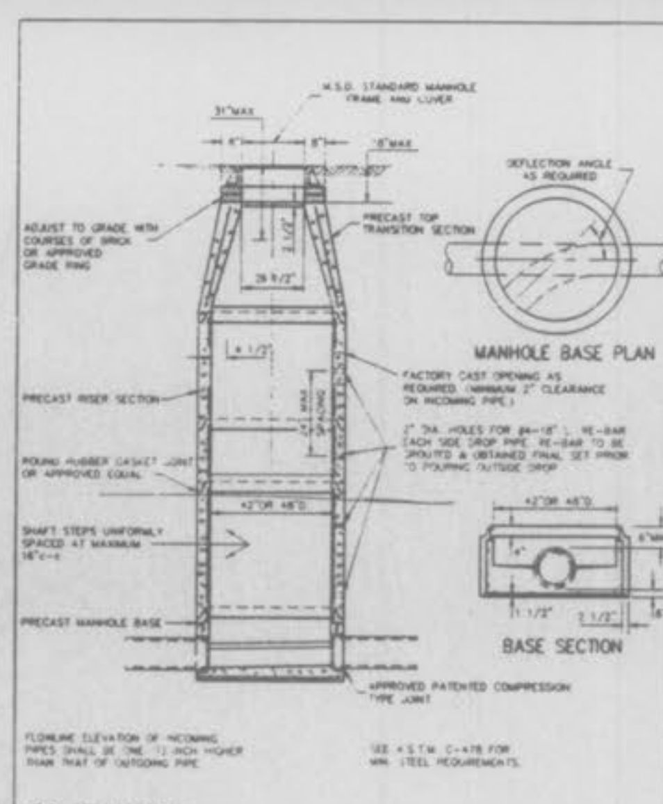
PRE-CAST CONCRETE MANHOLE FOR SEWERS 8" THROUGH 18" METROPOLITAN ST. LOUIS SEWER DISTRICT Standard Details of Sewer Construction
