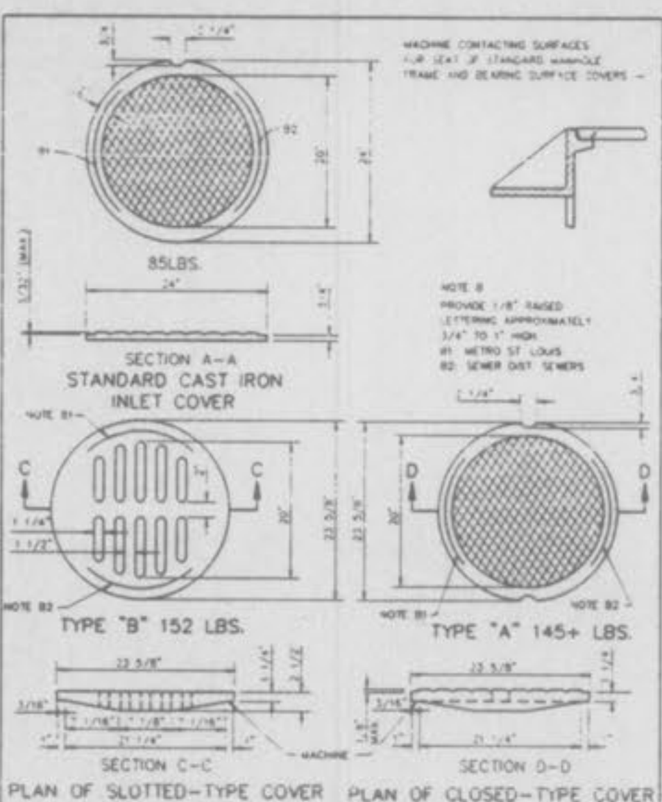
CAST IRON COVERS AND INLETS METROPOLITAN ST. LOUIS SEWER DISTRICT Standard Details of Sewer Construction
