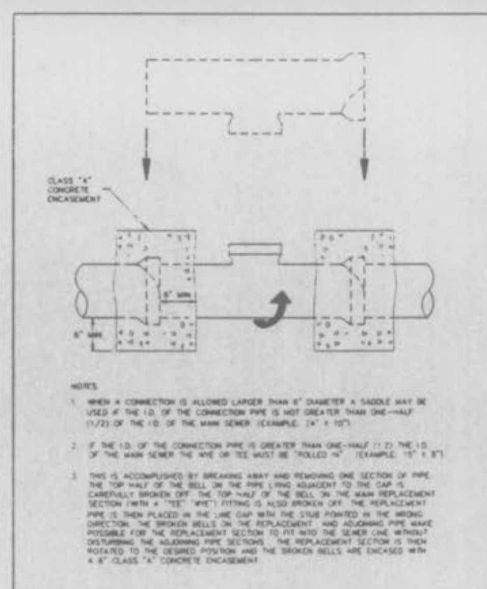
'ROLL-IN' (FOR EXISTING CLAY OR CONCRETE PIPE) METROPOLITAN ST. LOUIS SEWER DISTRICT Standard Details of Sewer Construction
