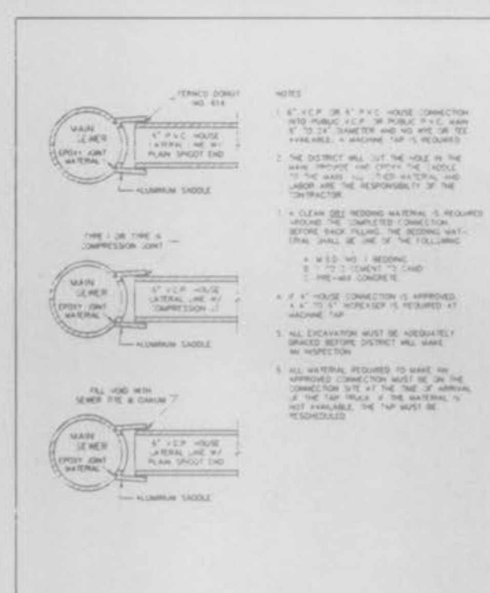
MACHINE TAP METROPOLITAN ST. LOUIS SEWER DISTRICT Standard Details of Sewer Construction
