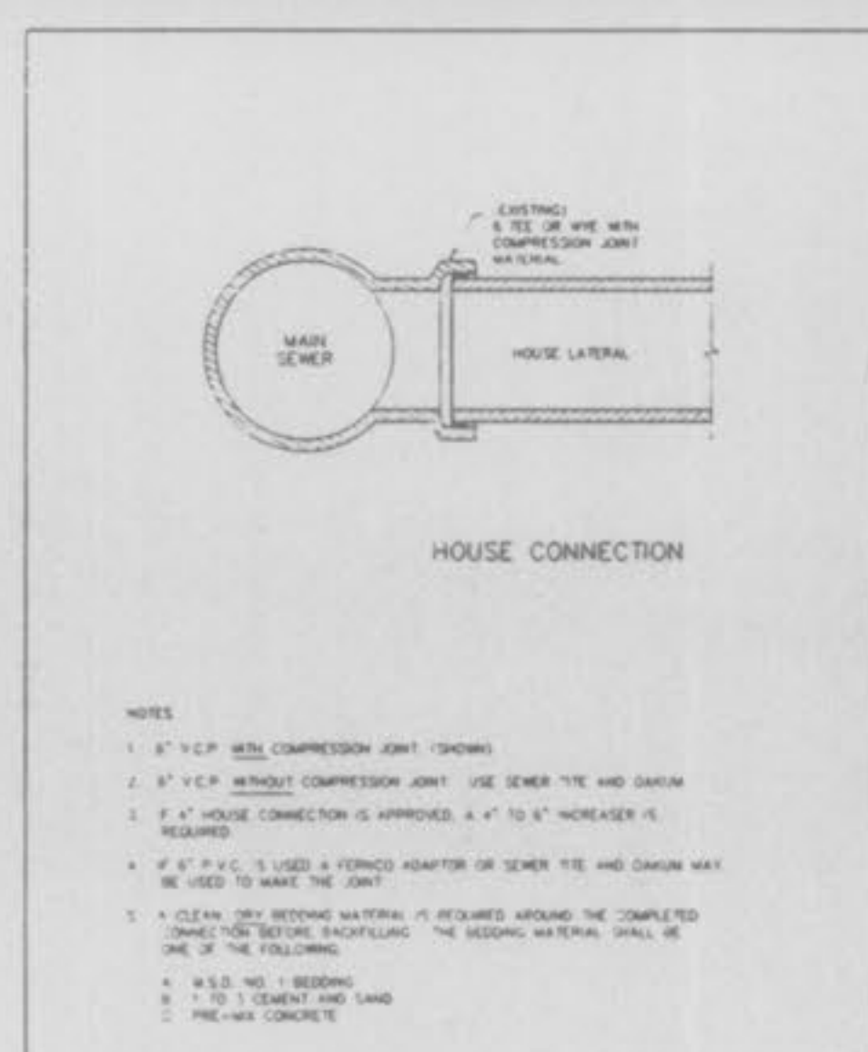
HOUSE CONNECTION TO EXISTING TEE OR WYE METROPOLITAN ST. LOUIS SEWER DISTRICT Standard Details of Sewer Construction
