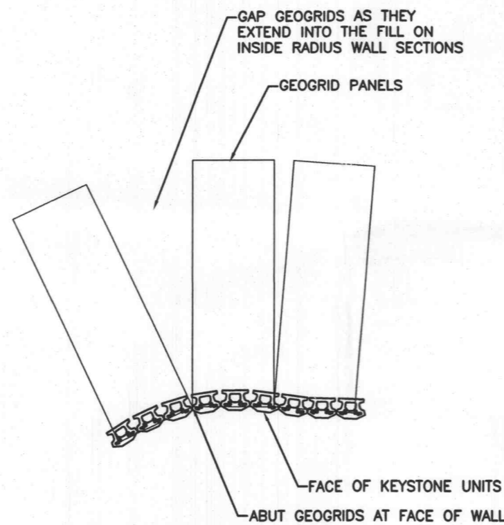
INSIDE RADIUS DETAIL NOT TO SCALE
