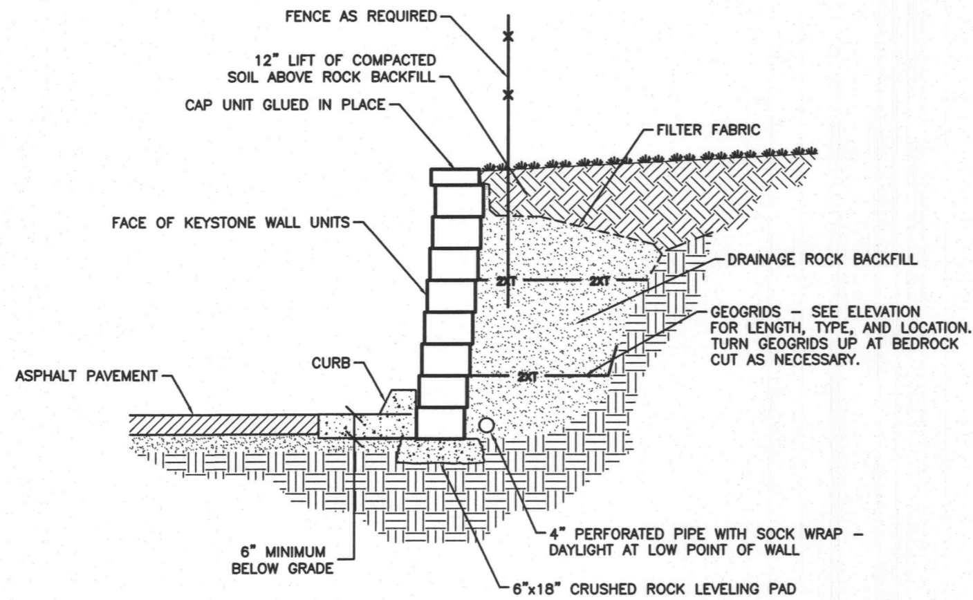
TYPICAL SECTION NOT TO SCALE
