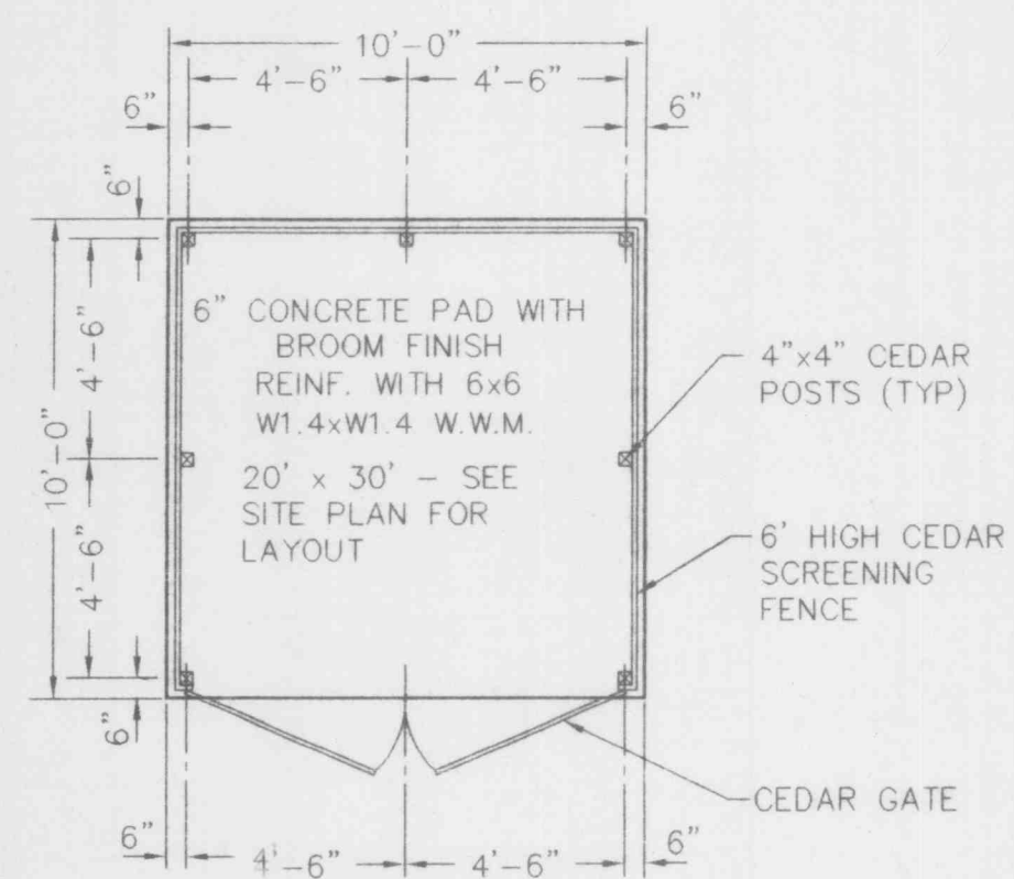
TRASH ENCLOSURE/PAD NOT TO SCALE
