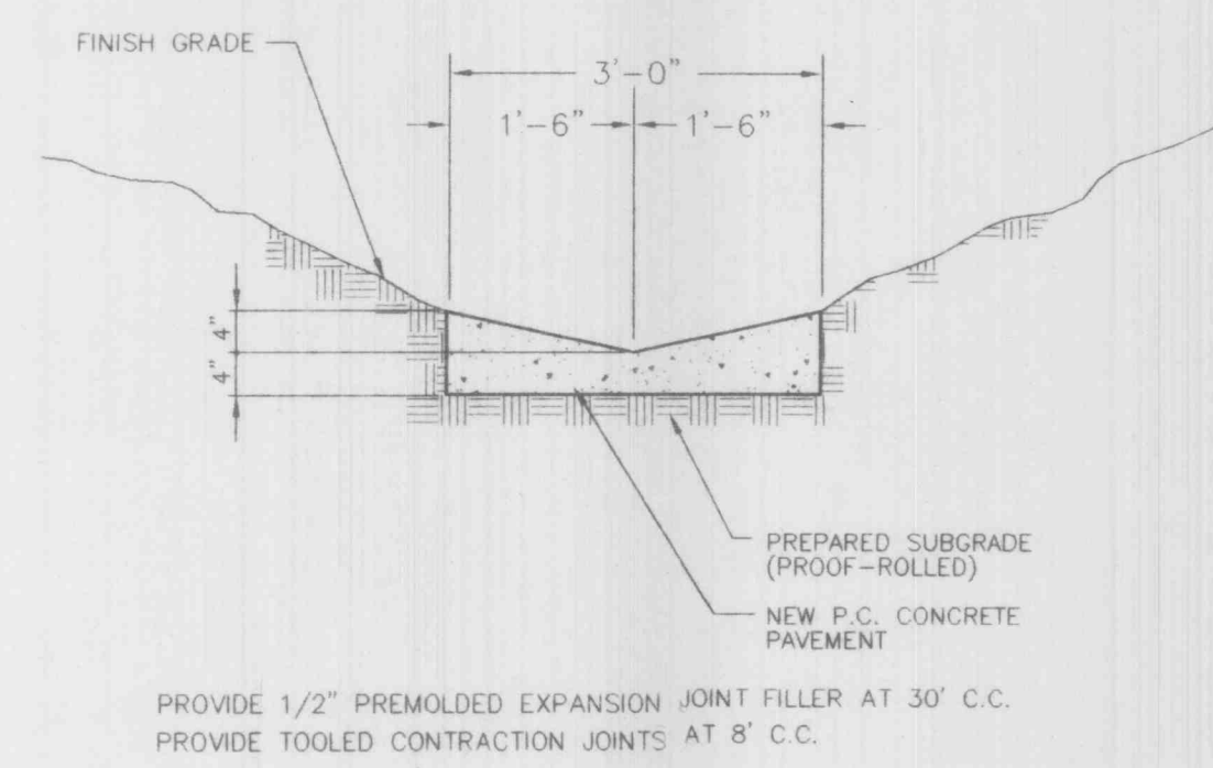
CONCRETE SWALE NOT TO SCALE
