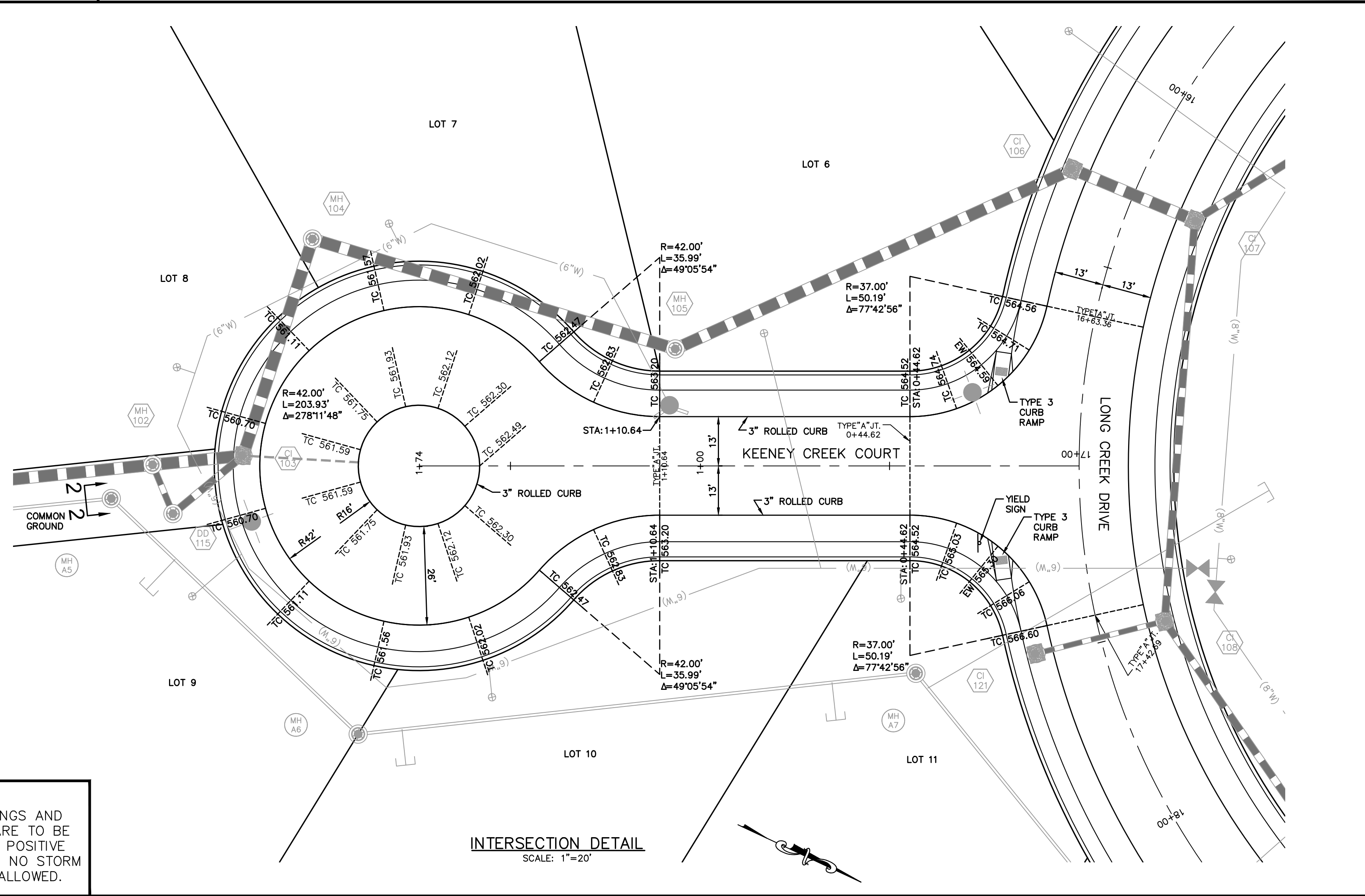
INTERSECTION DETAIL SCALE: 1"=20'
