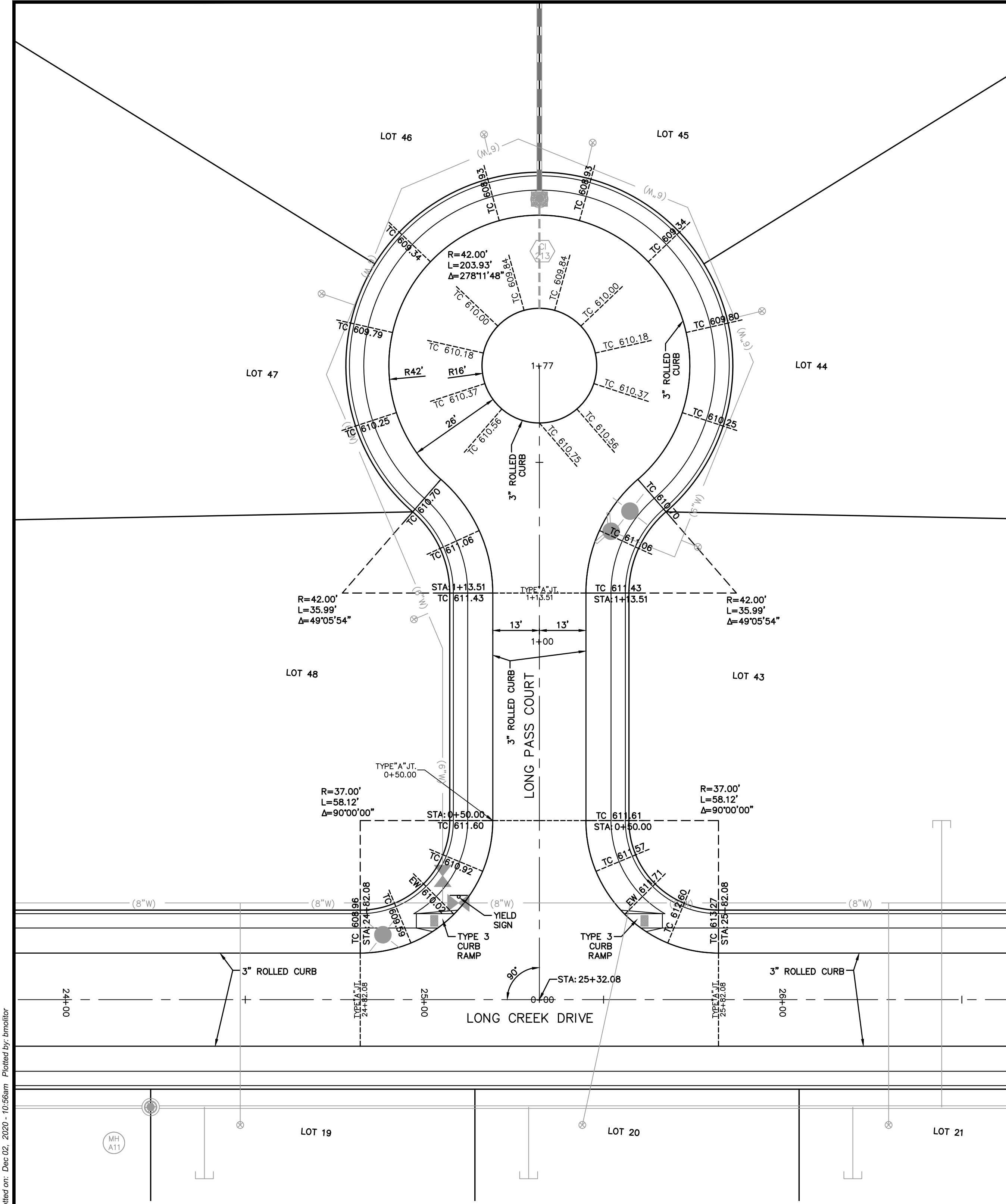
INTERSECTION DETAIL SCALE: 1"=20'
