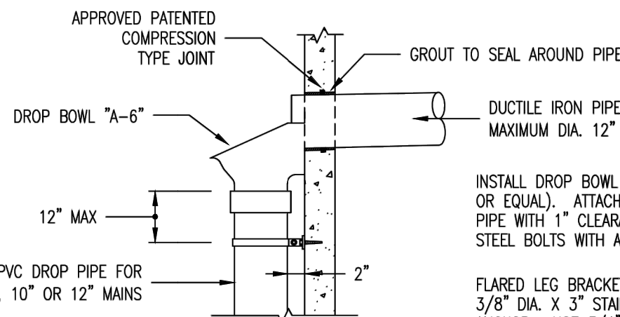
DETAIL "A" STANDARD DROP PIPE
