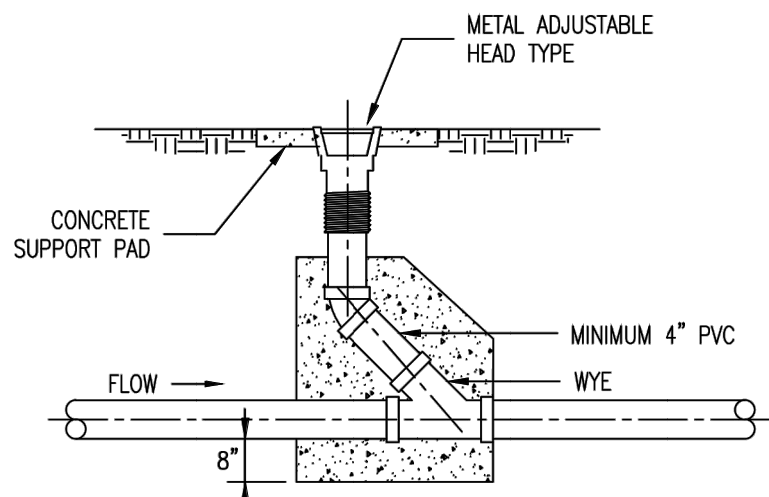
ADJUSTABLE HEAD TYPE CLEANOUT
