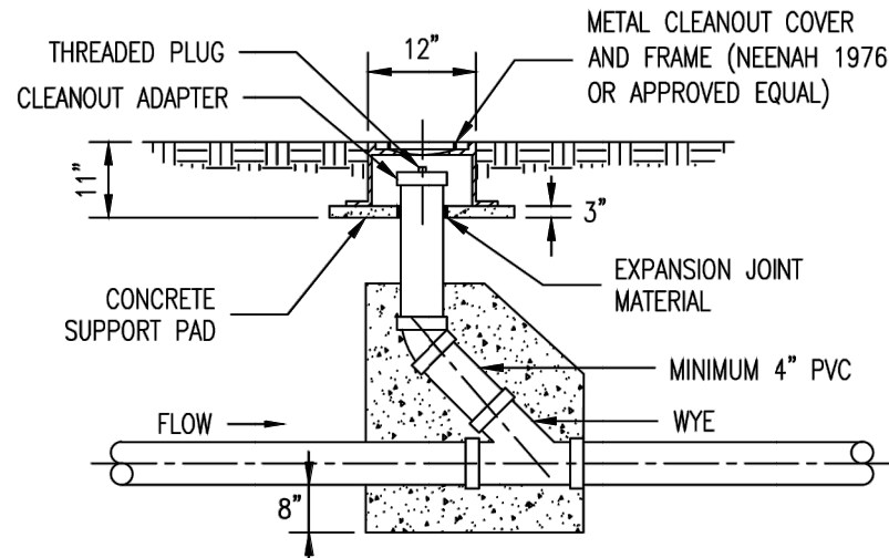
METAL FRAME AND COVER TYPE CLEANOUT
