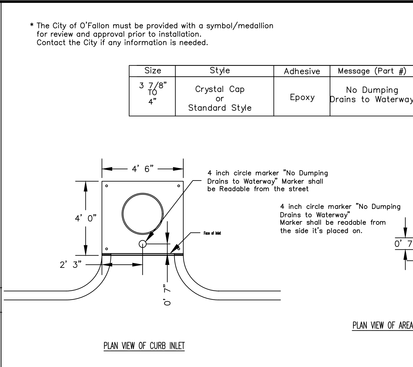
CITY OF O'FALLON ENGINEERING DEPARTMENT O'FALLON, MISSOURI SEWER CONSTRUCTION DETAILS FLARED END SECTION (INLET/OUTLET PROTECTION)
