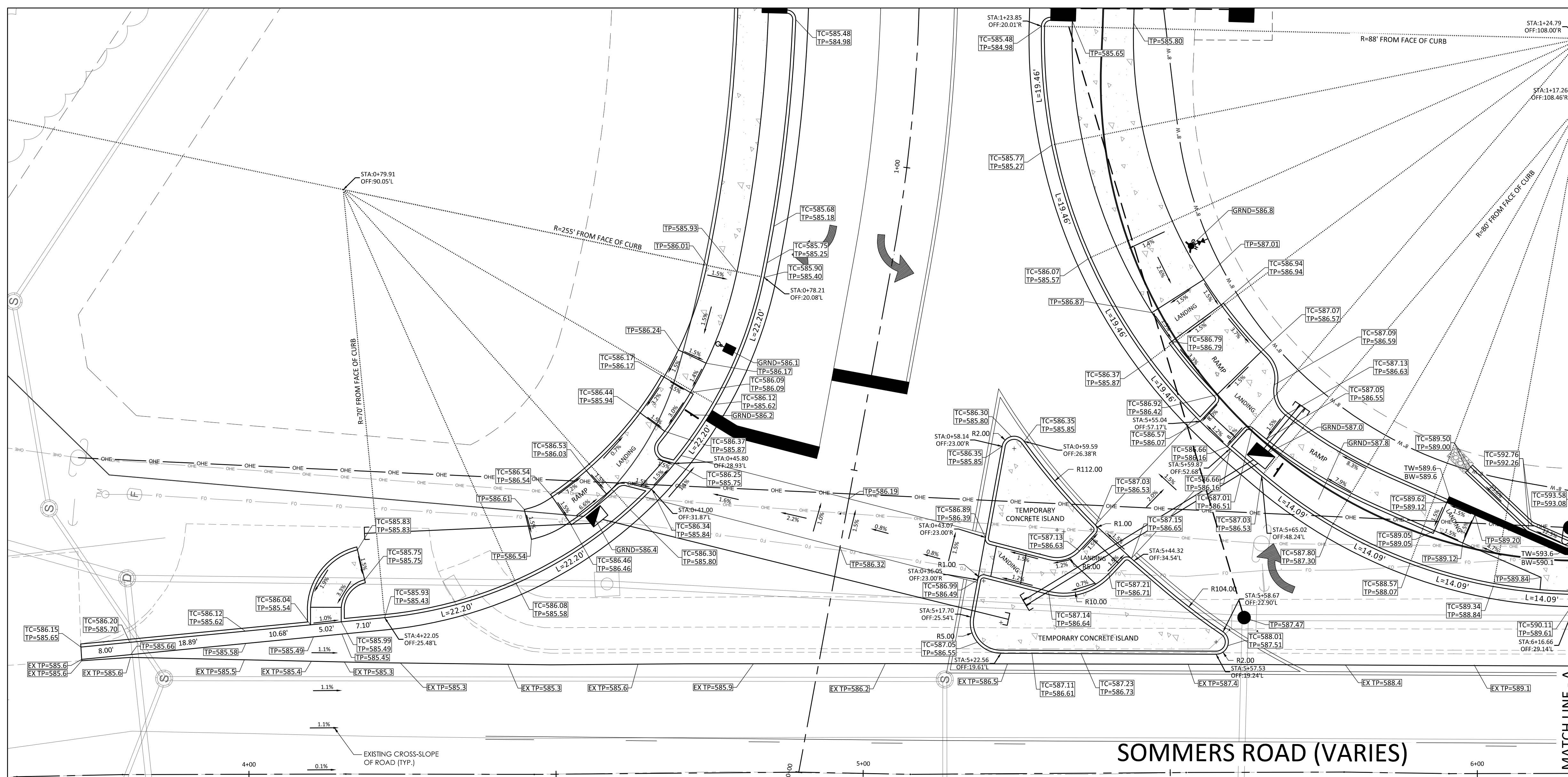
1A HANDICAP RAMP AND WARPING DETAIL SCALE: 1"=10'
