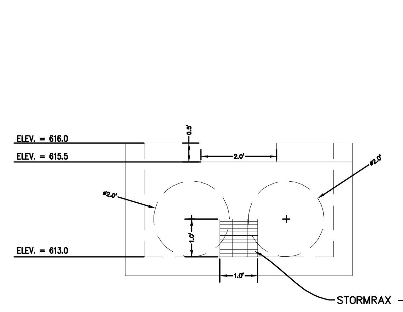
OUTLET STRUCTURE ELEVATION VIEW
