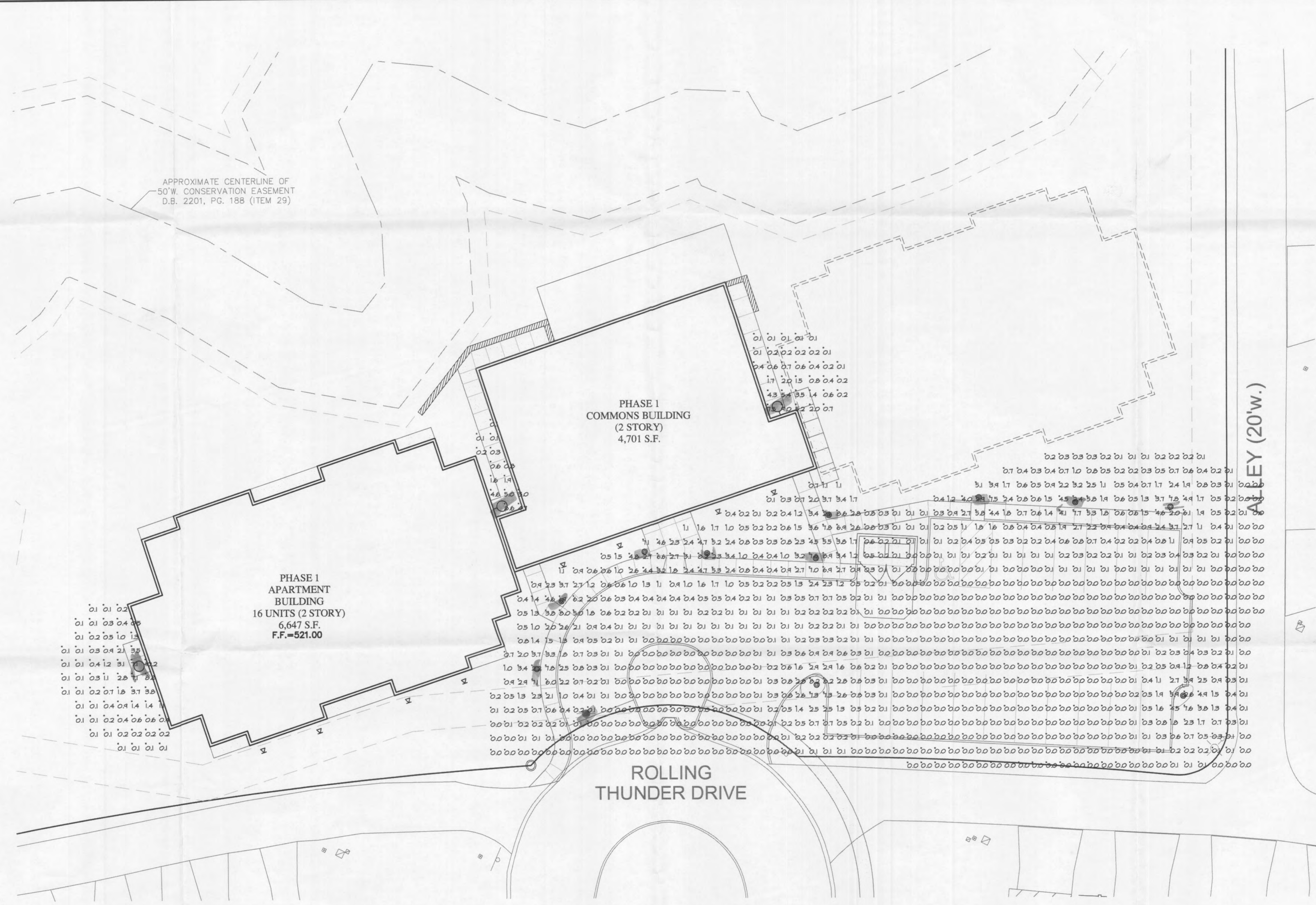
SITE PLAN - PHOTOMETRIC SCALE: 1/16" = 1'-0"
