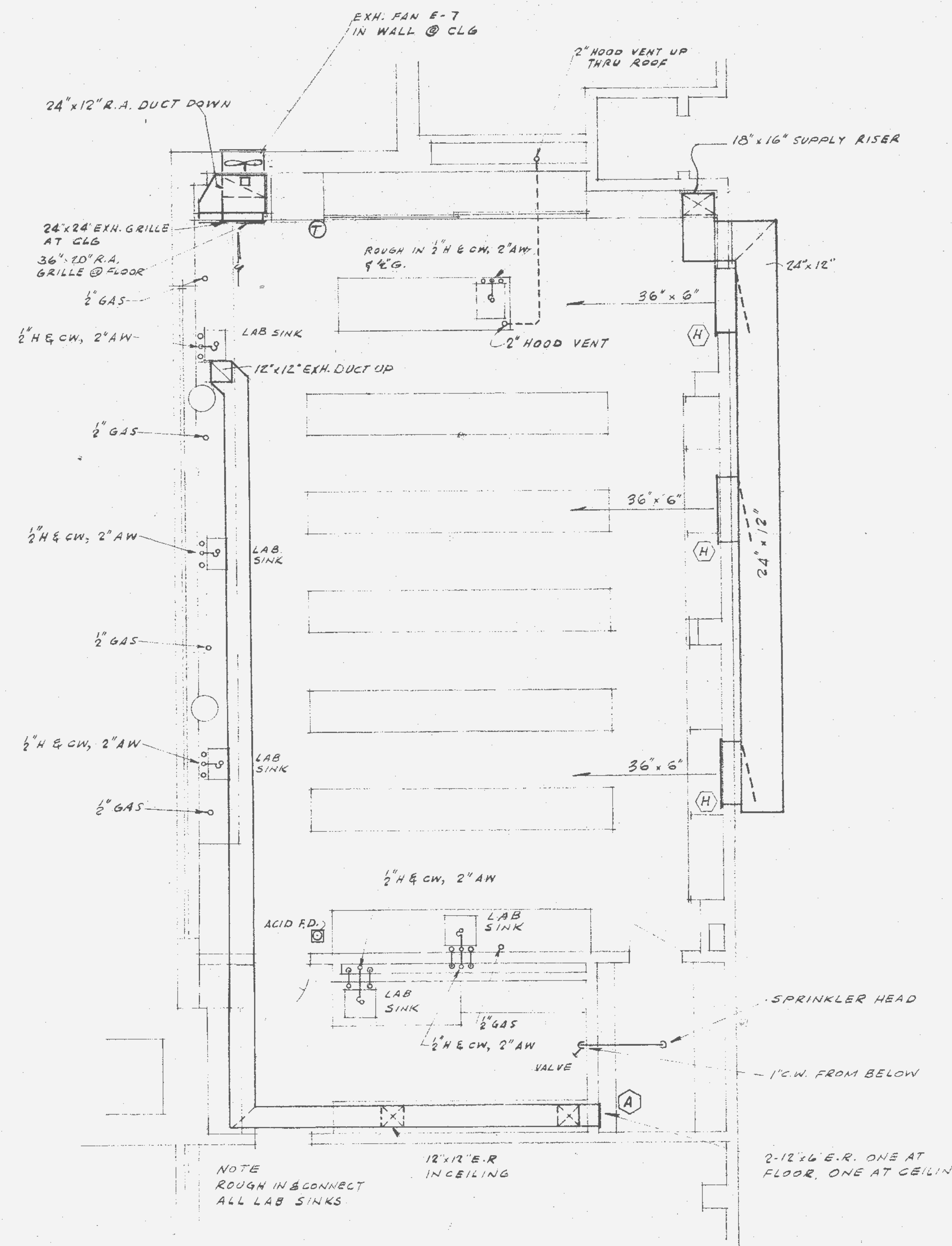
PLAN OF SCIENCE LAB-113 SCALE: 1/4" = 1'-0"
