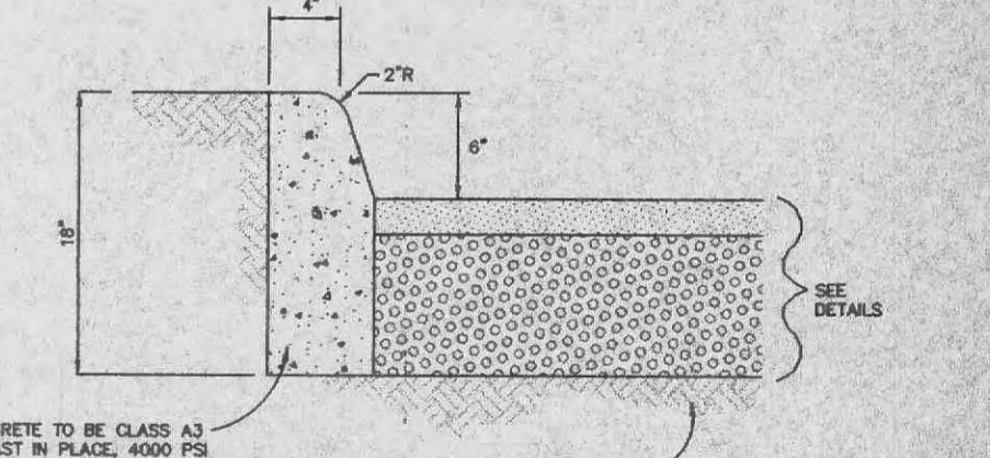
CONCRETE VERTICAL CURB DETAIL FOR ASPHALT PAVEMENT (n.t.s.)
