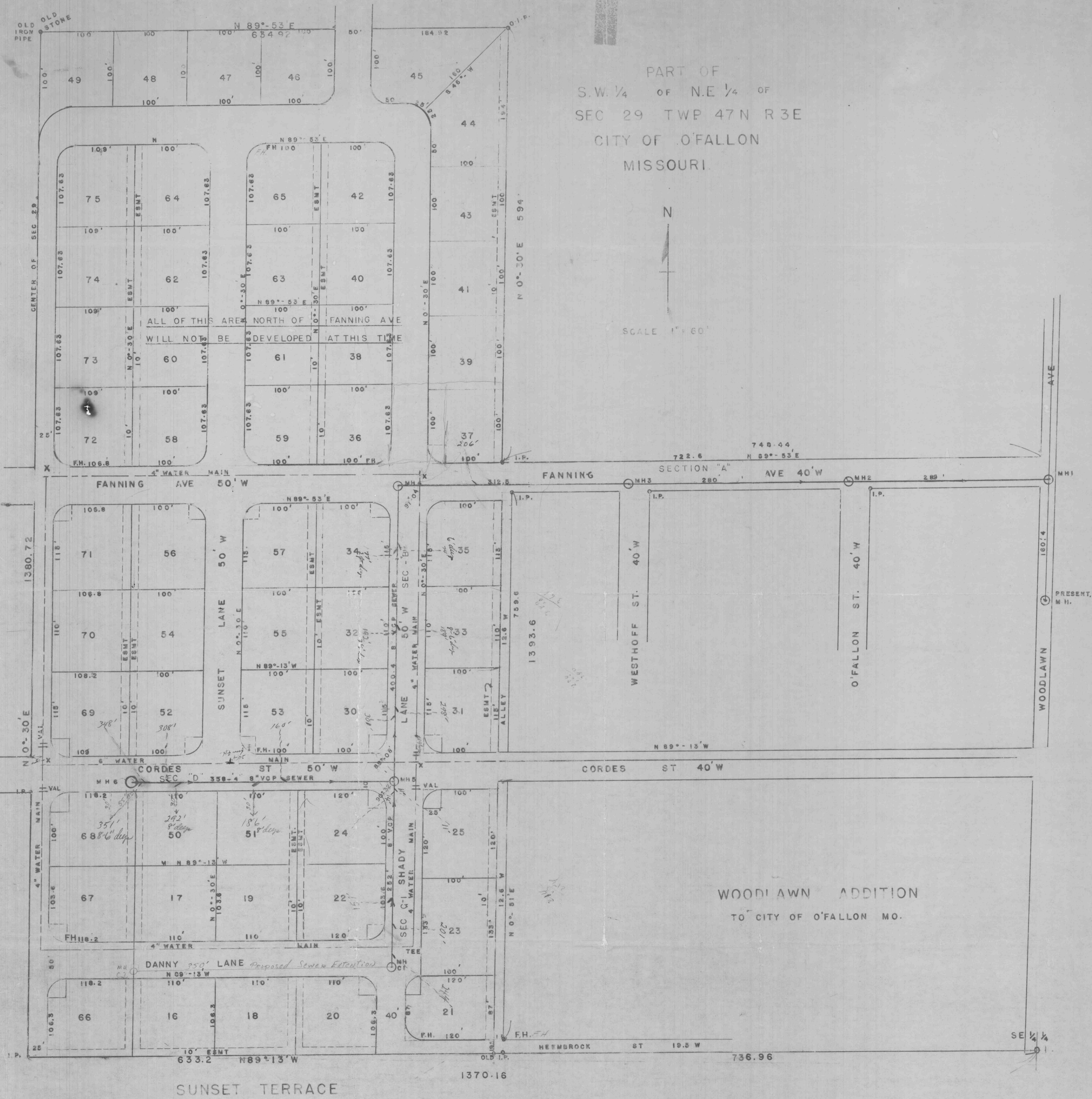
GENERAL LAYOUT PLAN FOR SEWER & WATER EXTENSIONS
