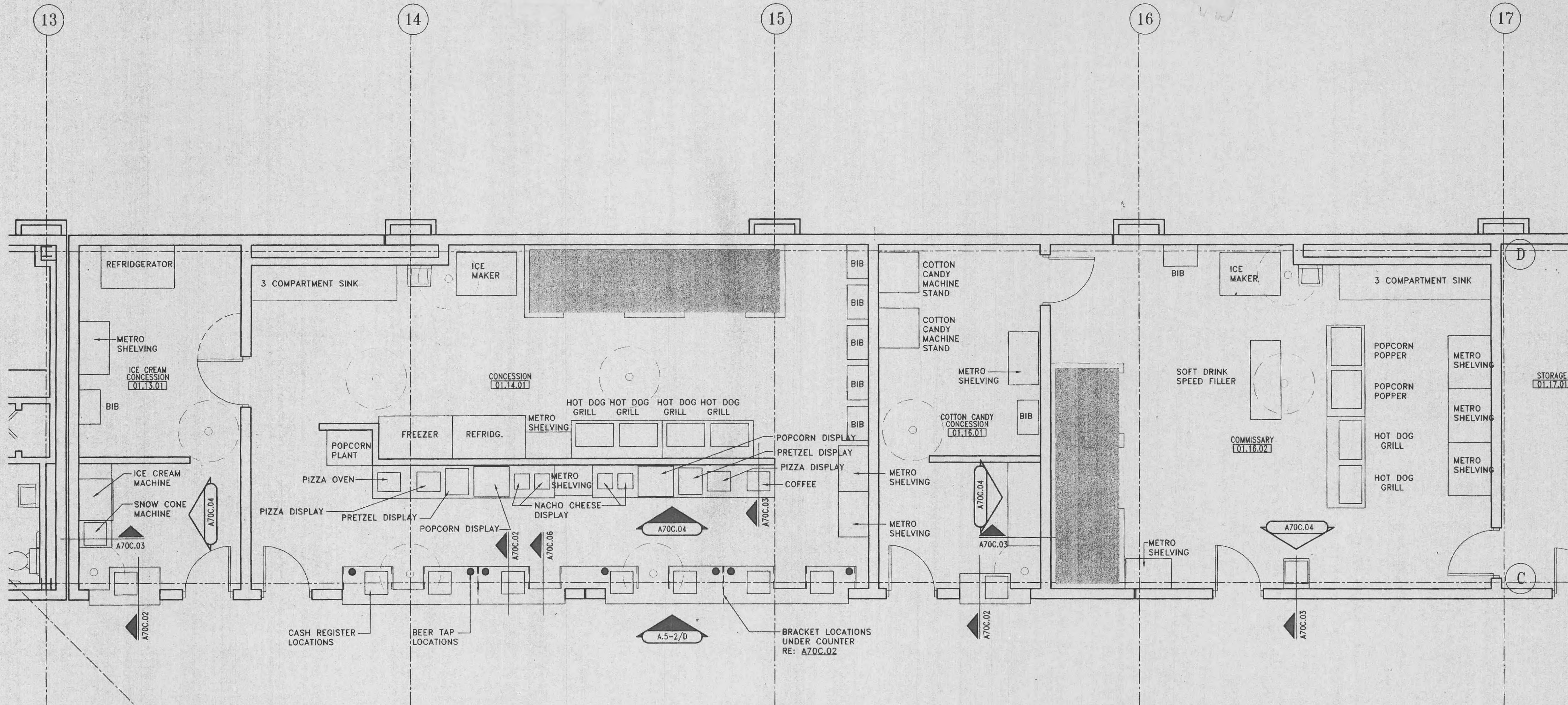
A CONCESSION EQUIPMENT LAYOUT 1/4" = 1'-0"
