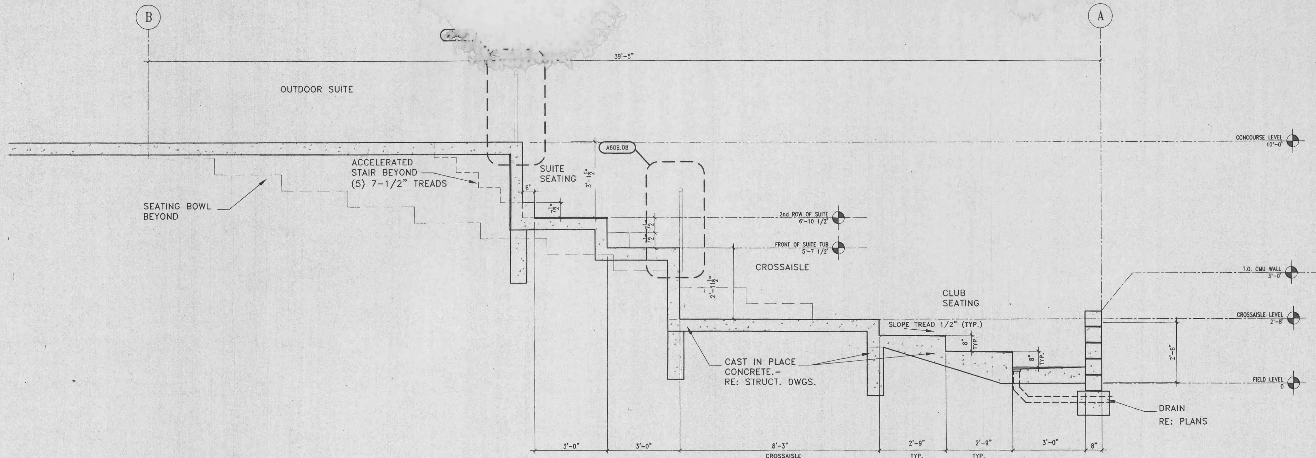
A ENLARGED SECTION @ SUITE / CLUB SEATING 1/2"=1'-0"
