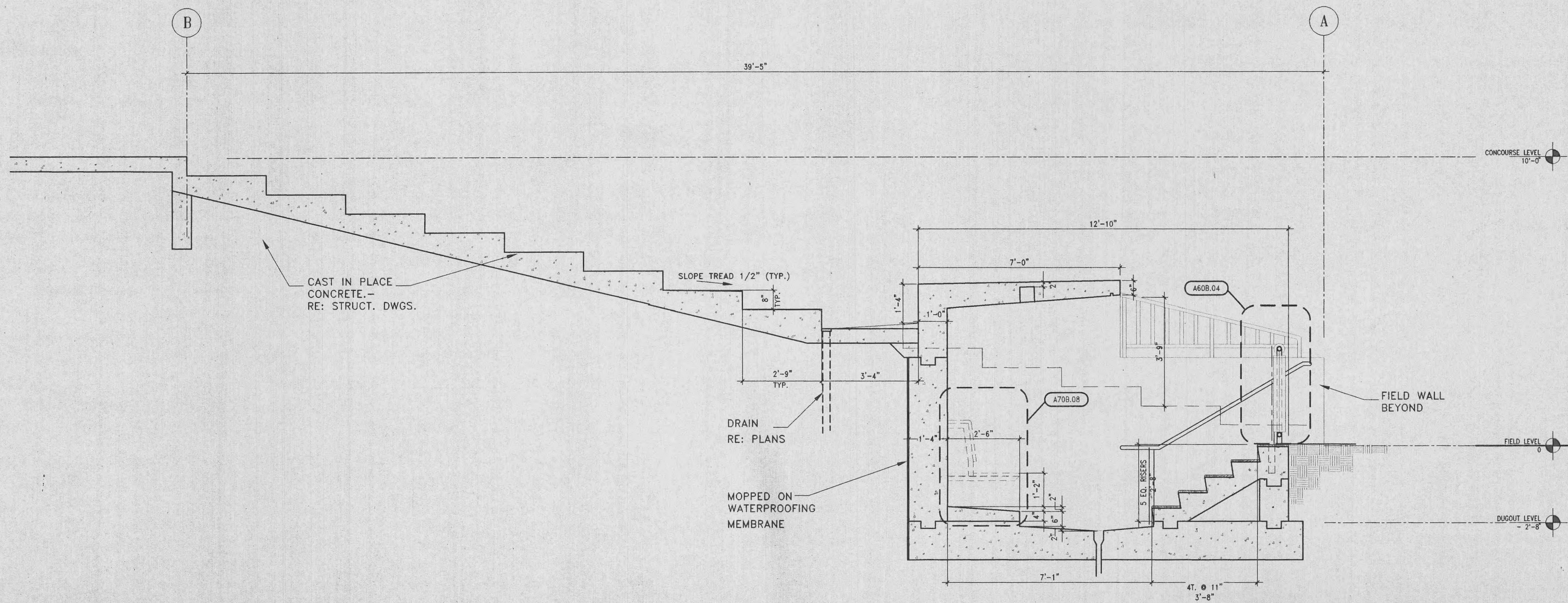
B ENLARGED SECTION @ DUGOUT 1/2"=1'-0"
