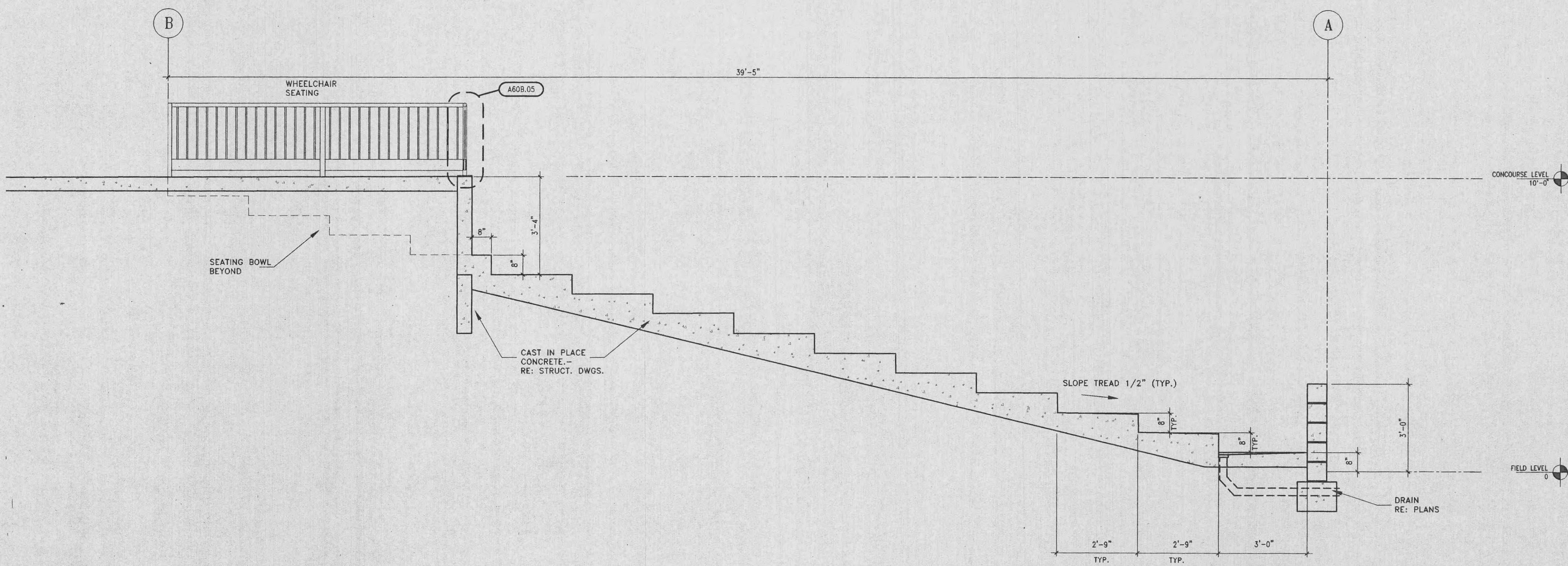
B ENLARGED SECTION @ THIRD BASE 1/2" = 1'-0"
