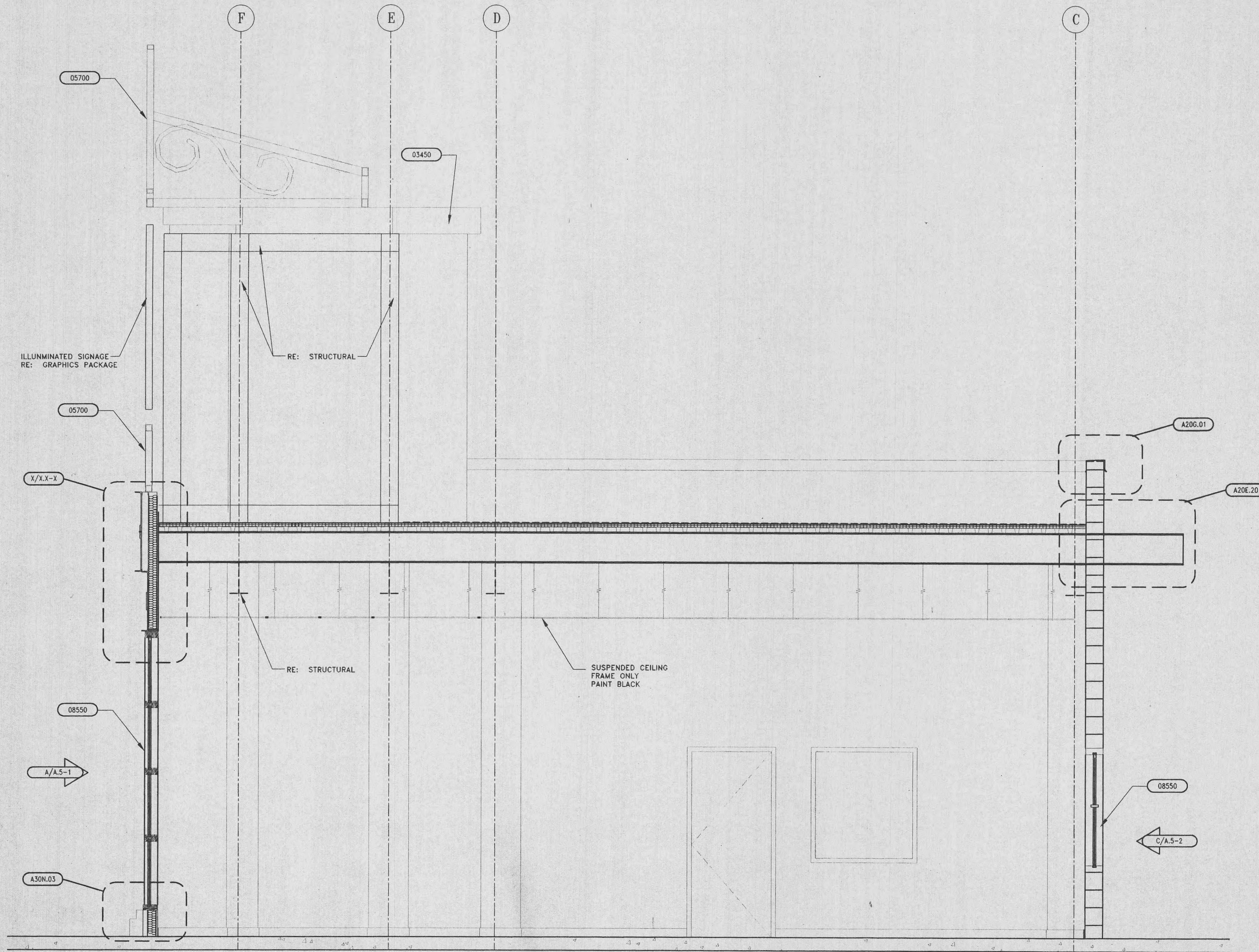
a SECTION @ HALL OF FAME WINDOWS 1/2" = 1'-0"
