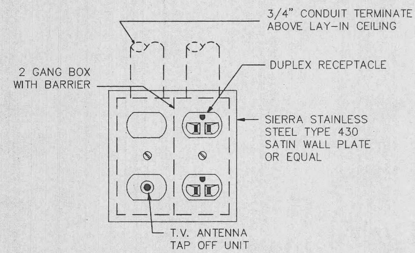
T.V. OUTLET DETAIL NOT TO SCALE
