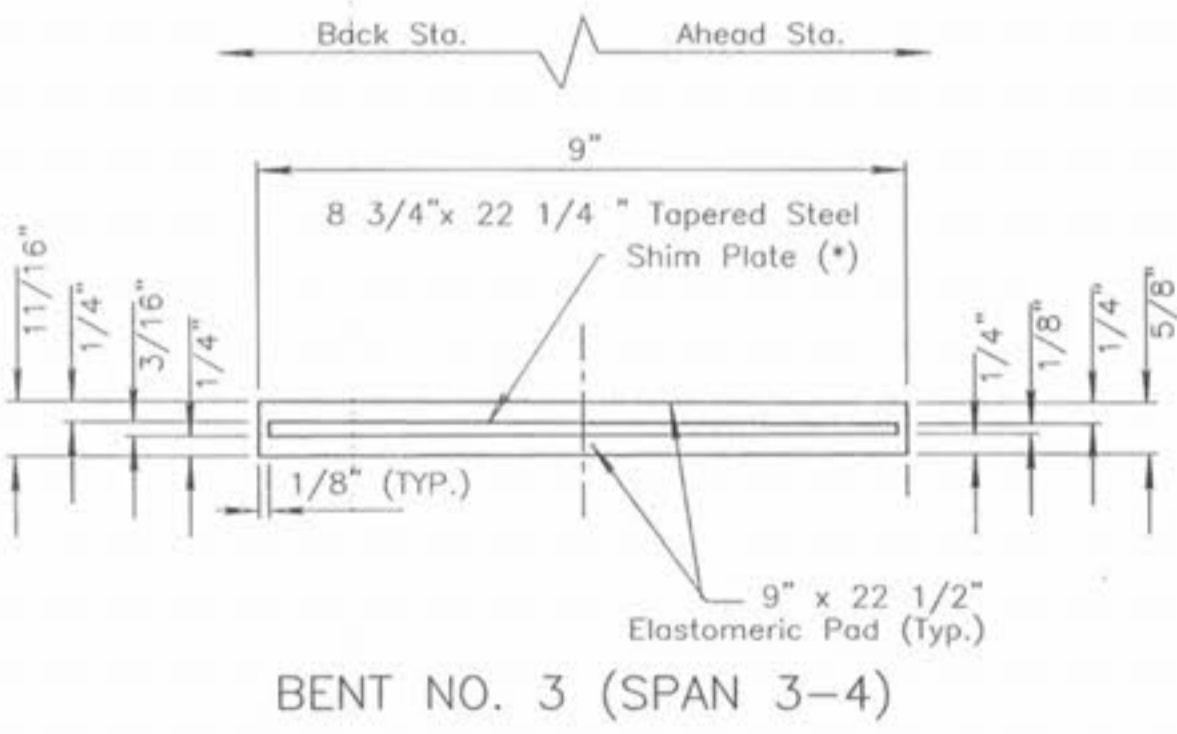
DETAIL OF LAMINATED NEOPRENE BEARING PAD
