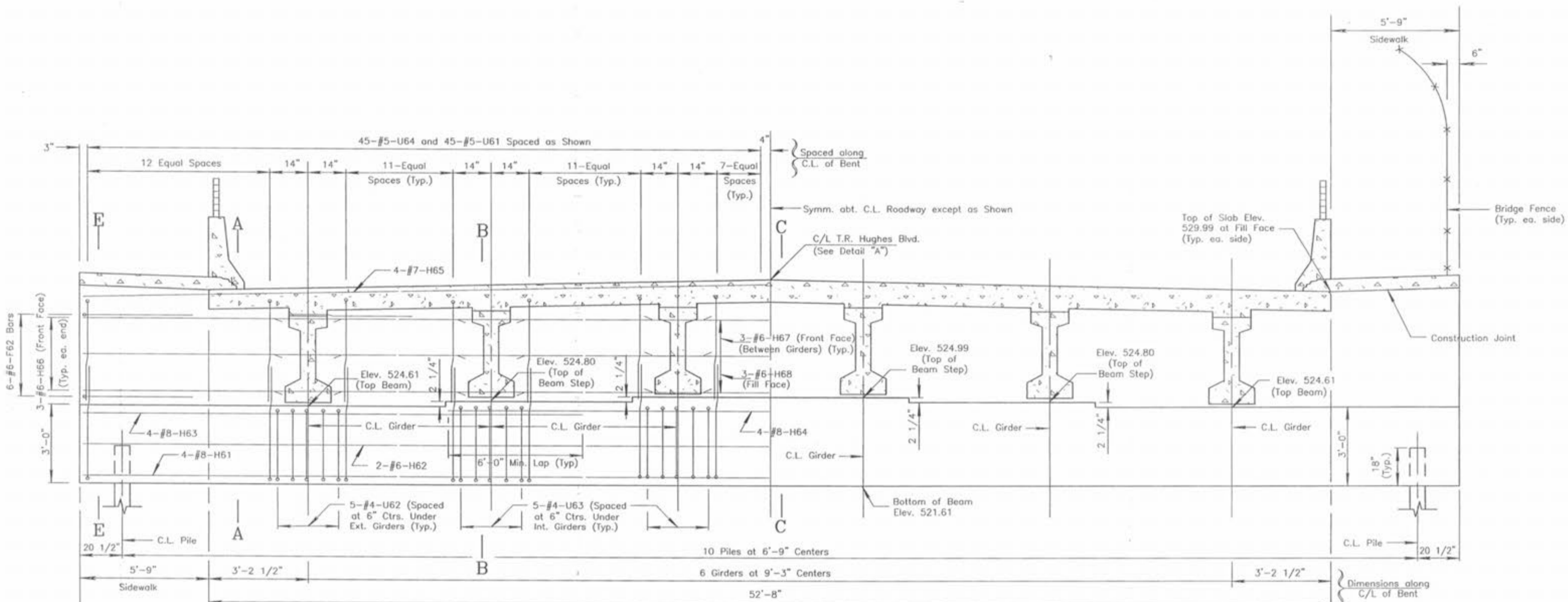
HALF SECTION NEAR END BENT (showing Reinforcement)
