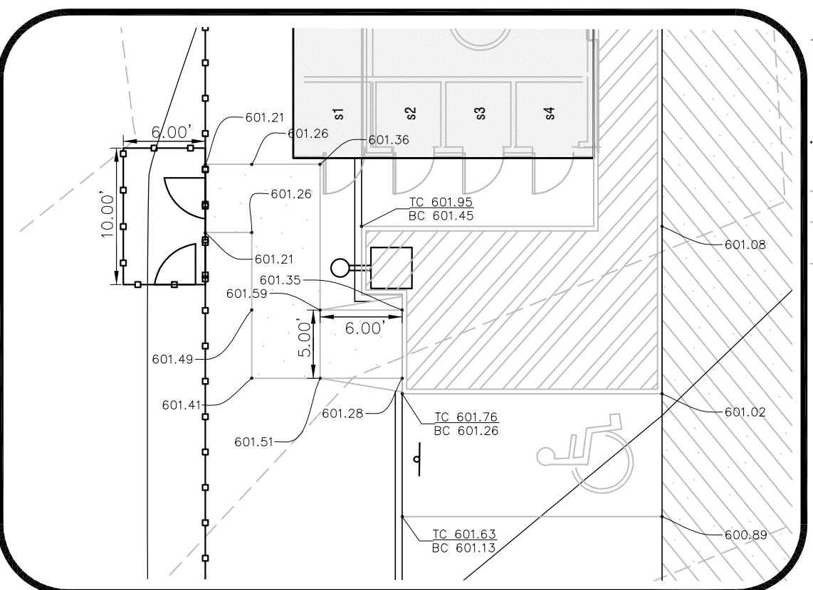
BARK PARK ENTRANCE DETAIL 1 INCH = 10 FEET
