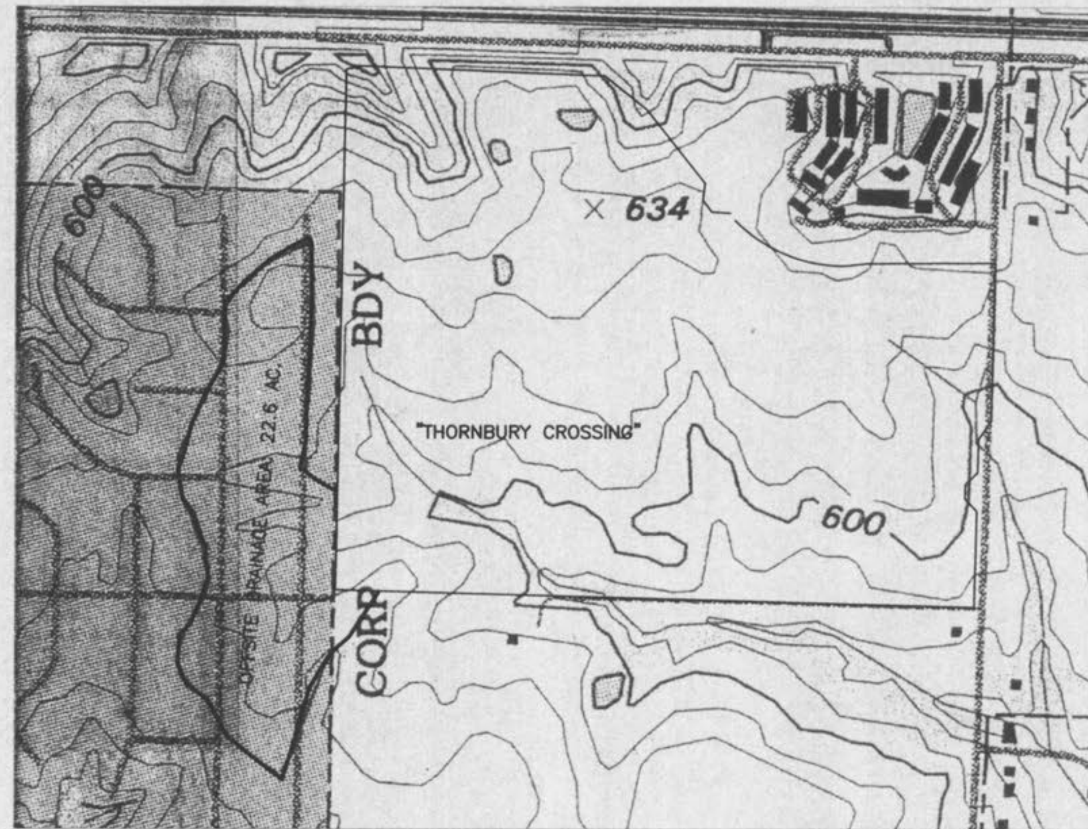
OFFSITE DRAINAGE AREA MAP SCALE: 1" = 400'
