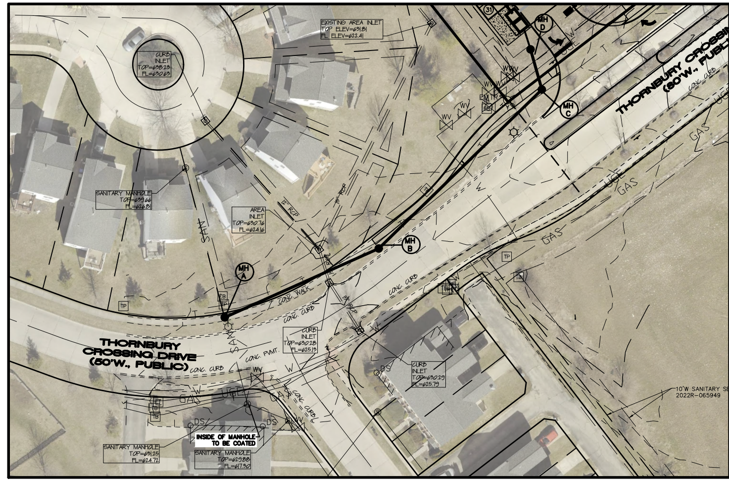
PLAN VIEW SCALE: 1"=60'
