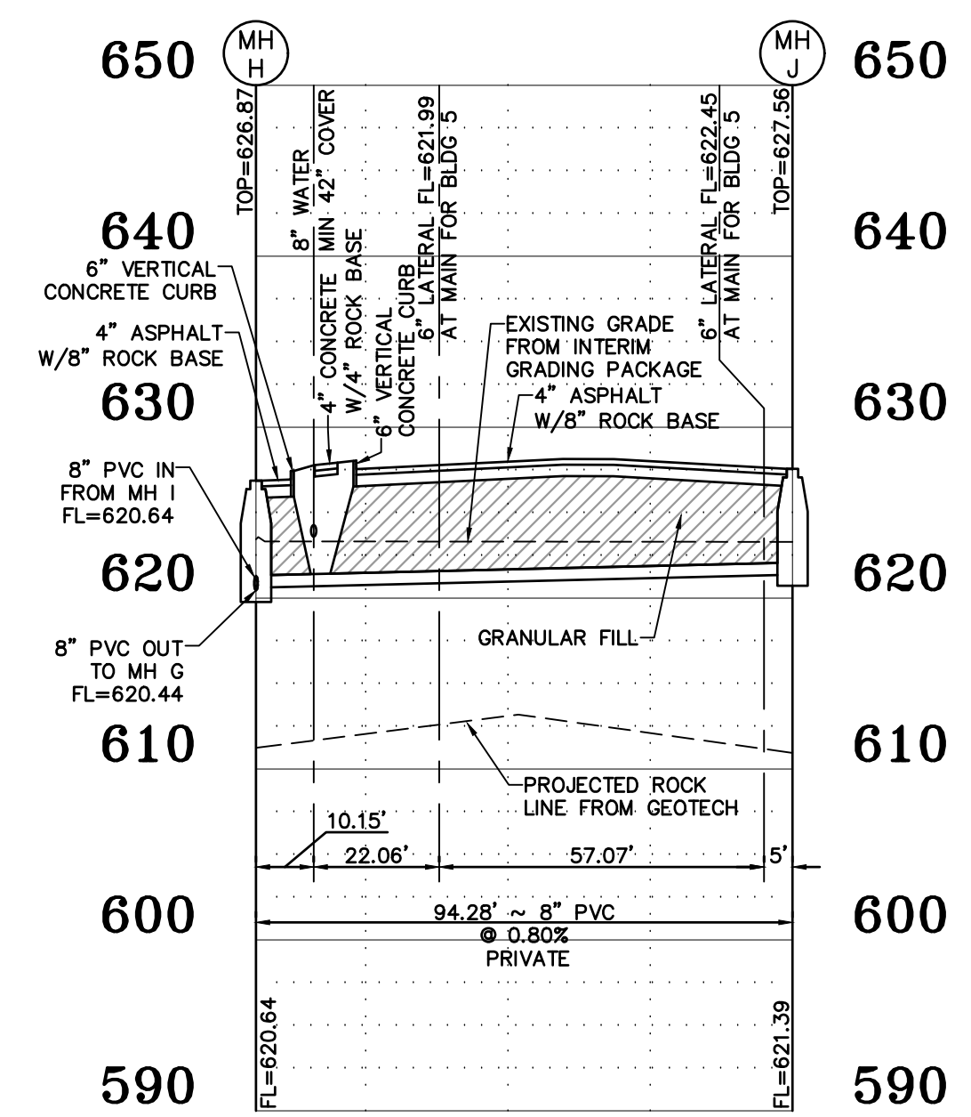
SANITARY PROFILE HORIZONTAL SCALE: 1"=30' VERTICAL SCALE: 1"=10'
