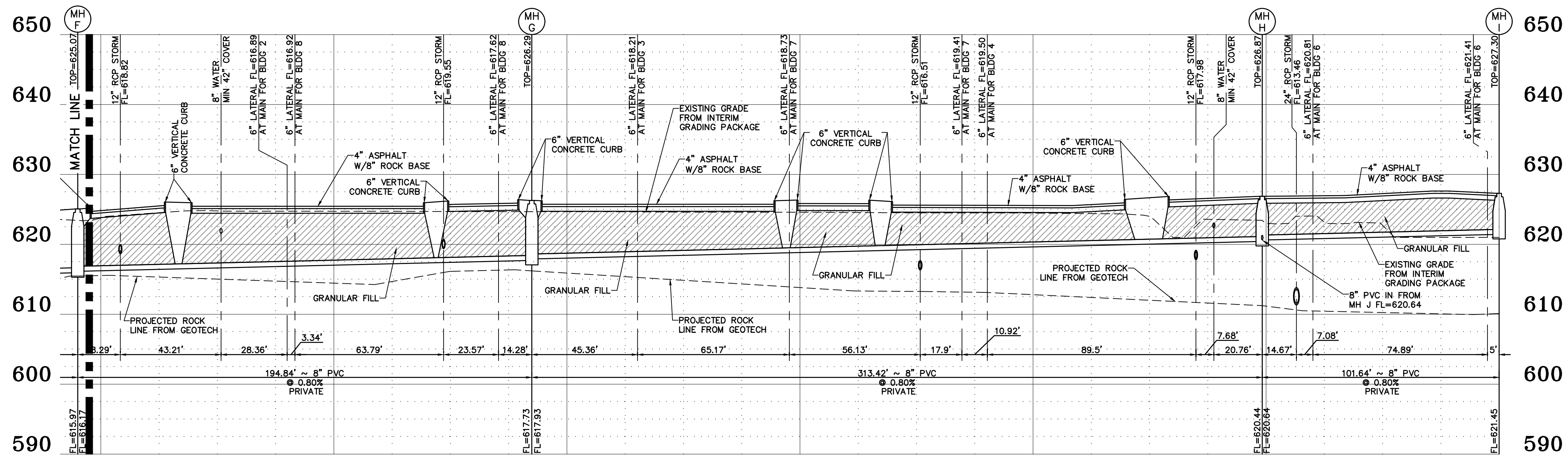
SANITARY PROFILE HORIZONTAL SCALE: 1"=30' VERTICAL SCALE: 1"=10'
