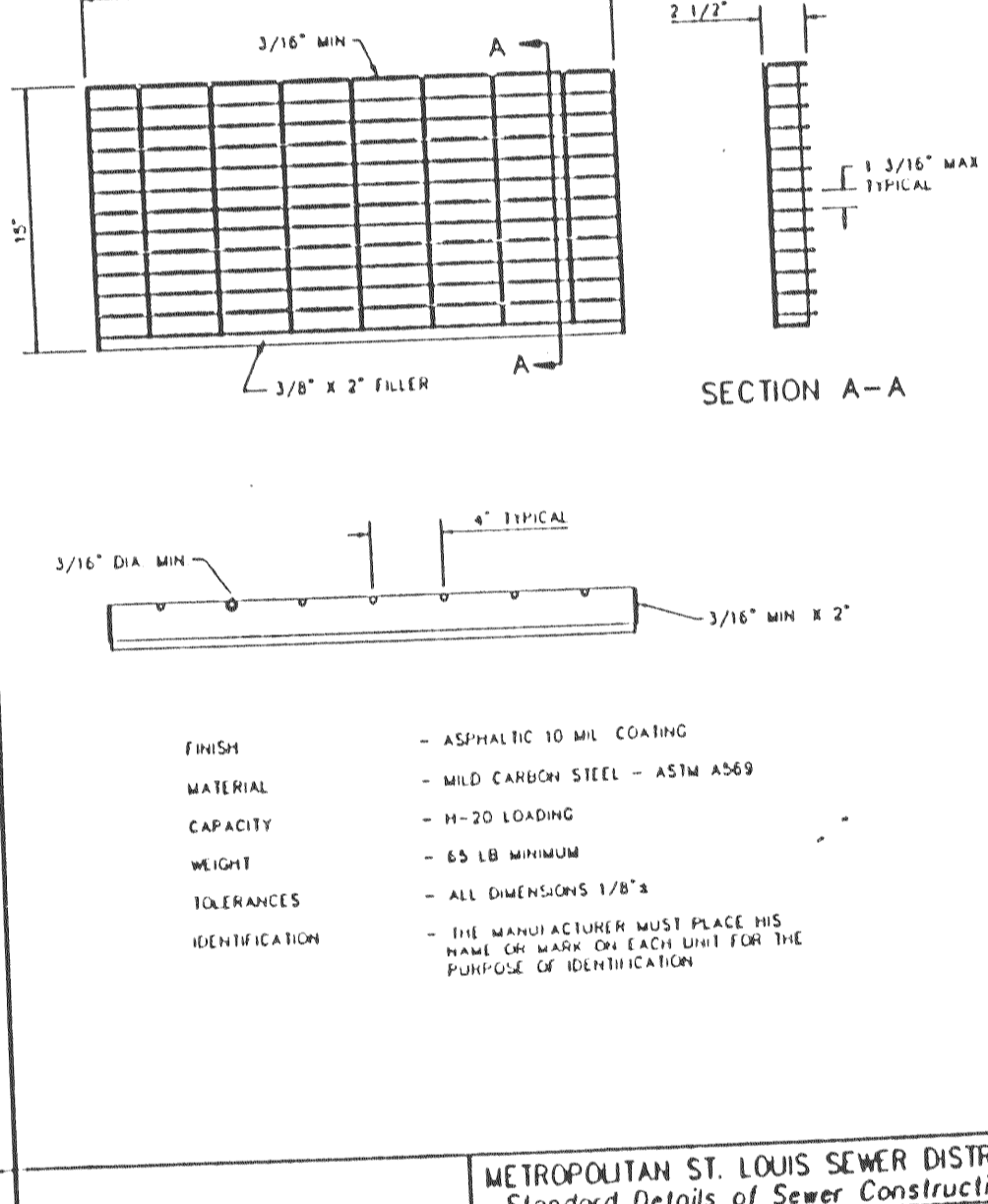
DETAIL OF STEEL GRATE METROPOLITAN ST. LOUIS SEWER DISTRICT Standard Details of Sewer Construction Dr. H.G.W. Ch. J.C.K. 1992 SHEET 45
