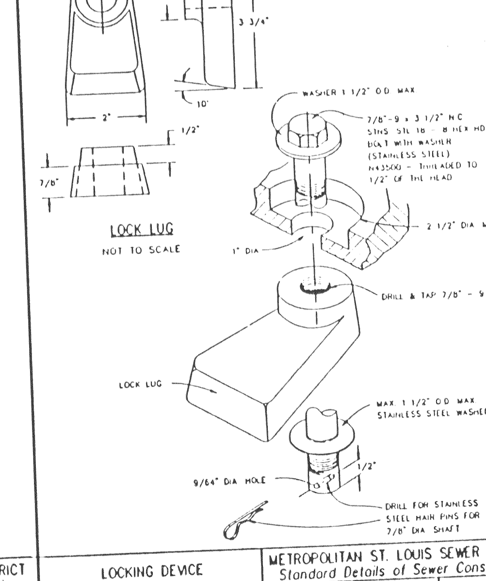
LOCKING DEVICE FOR TYPE 'N' LOCK TYPE MANHOLE COVER METROPOLITAN ST. LOUIS SEWER DISTRICT Standard Details of Sewer Construction Dr. J.E.G. Ch. J.C.K. 1992 SHEET 52
