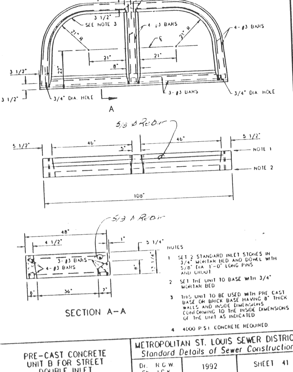
PRE-CAST CONCRETE UNIT B FOR STREET DOUBLE INLET METROPOLITAN ST. LOUIS SEWER DISTRICT Standard Details of Sewer Construction Dr. H.G.W. Ch. J.C.K. 1992 SHEET 41
