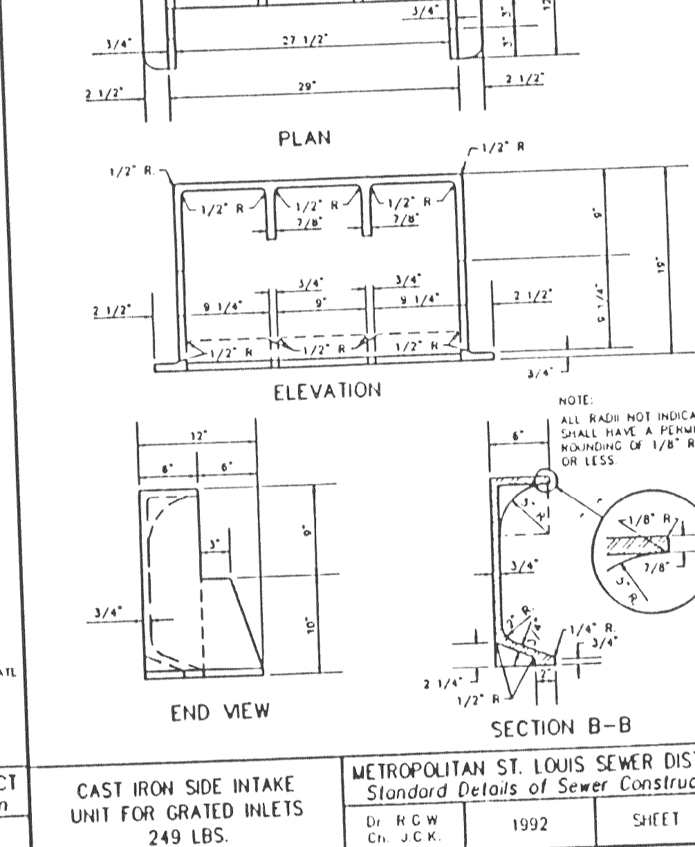
CAST IRON SIDE INTAKE UNIT FOR GRATED INLETS 249 LBS. METROPOLITAN ST. LOUIS SEWER DISTRICT Standard Details of Sewer Construction Dr. H.G.W. Ch. J.C.K. 1992 SHEET 47
