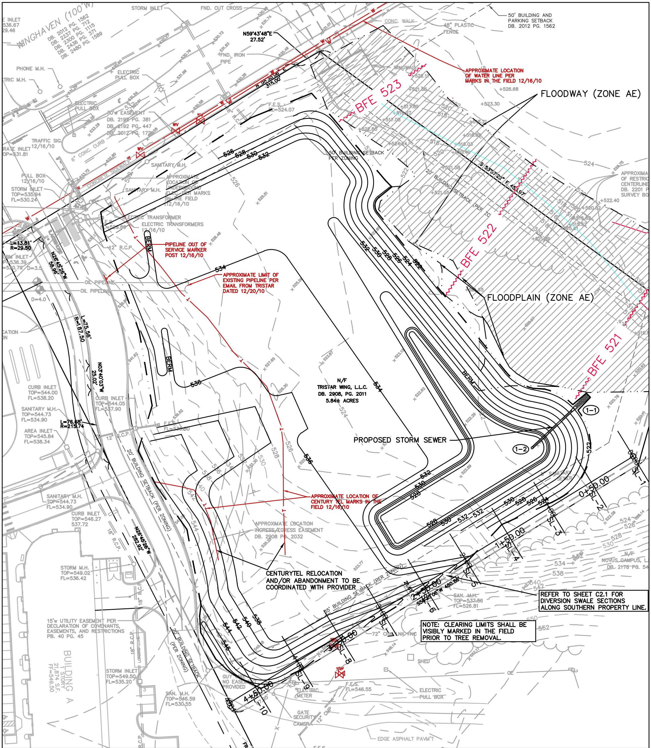
PROPOSED CONDITIONS PLAN SCALE: 1"=50'
