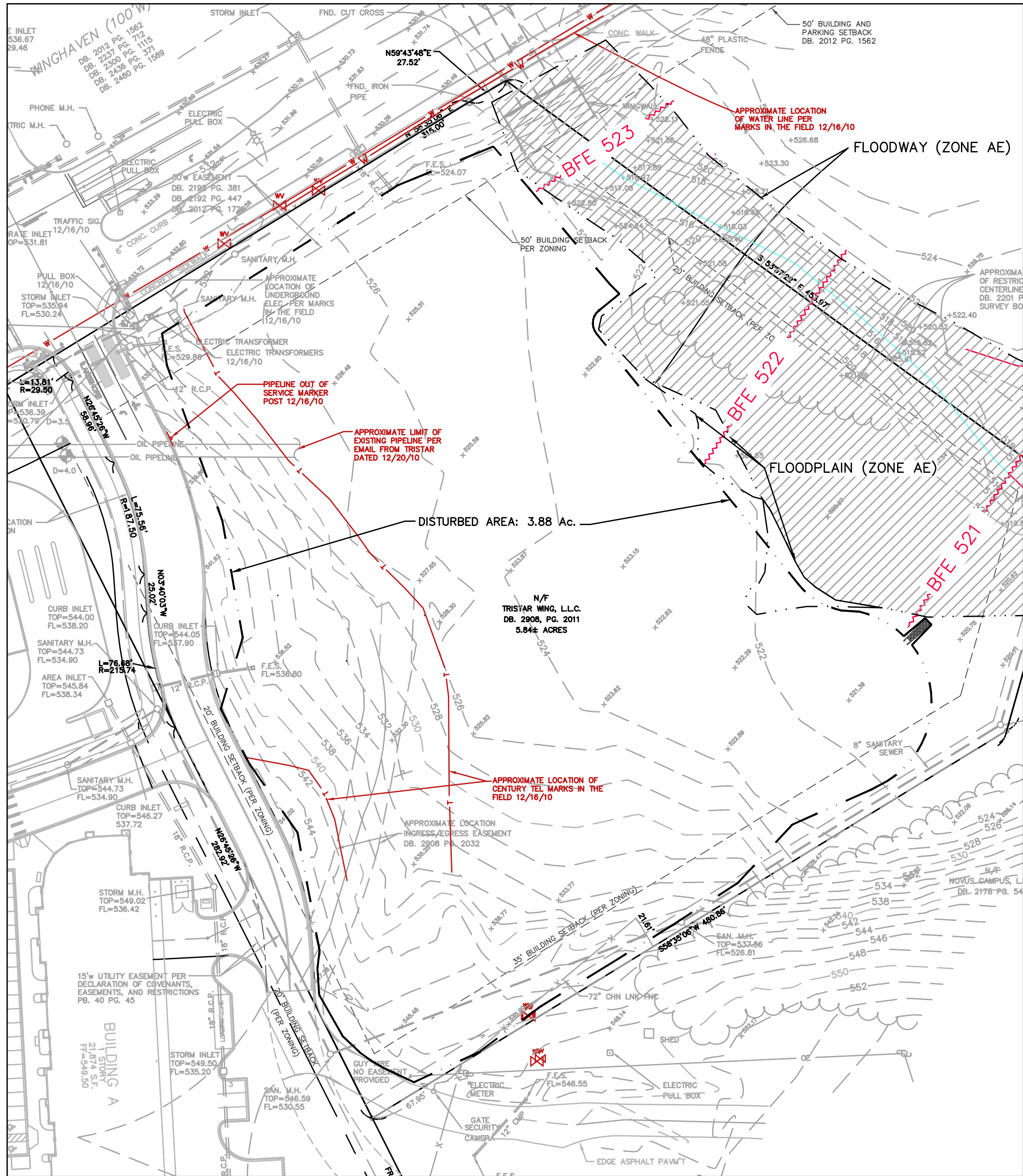
EXISTING CONDITIONS PLAN SCALE: 1"=50'
