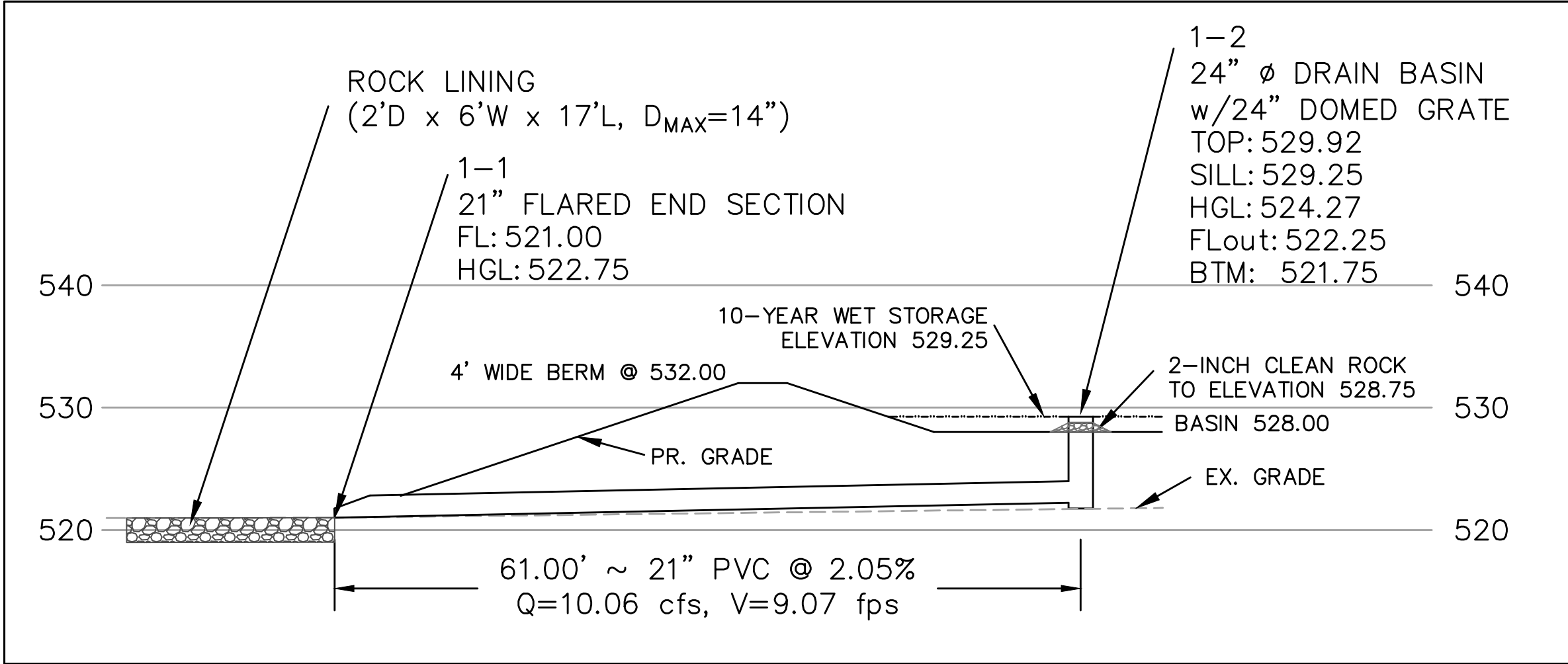
STORM SEWER PROFILE
