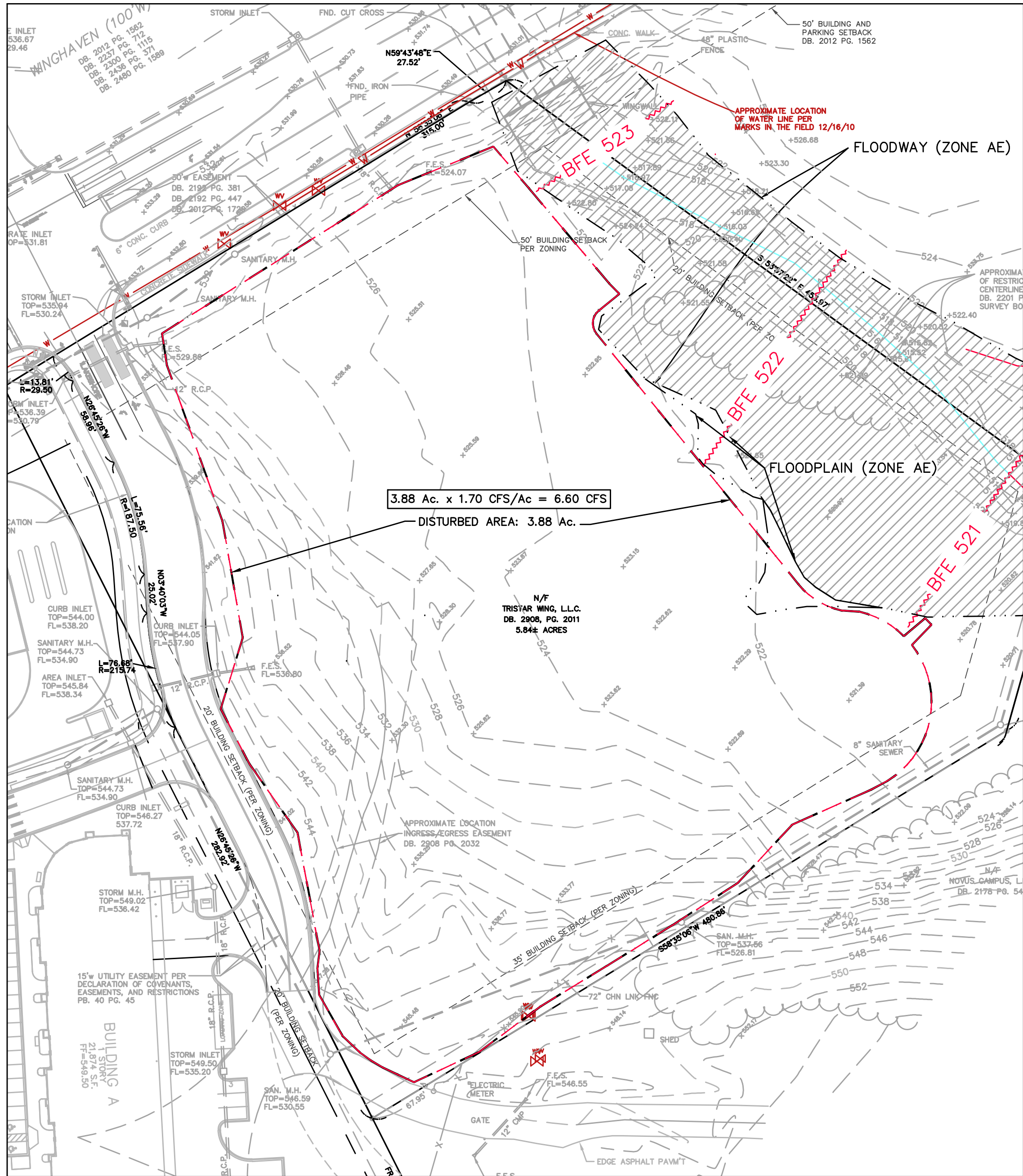
EXISTING DRAINAGE AREA MAP SCALE: 1"=50'
