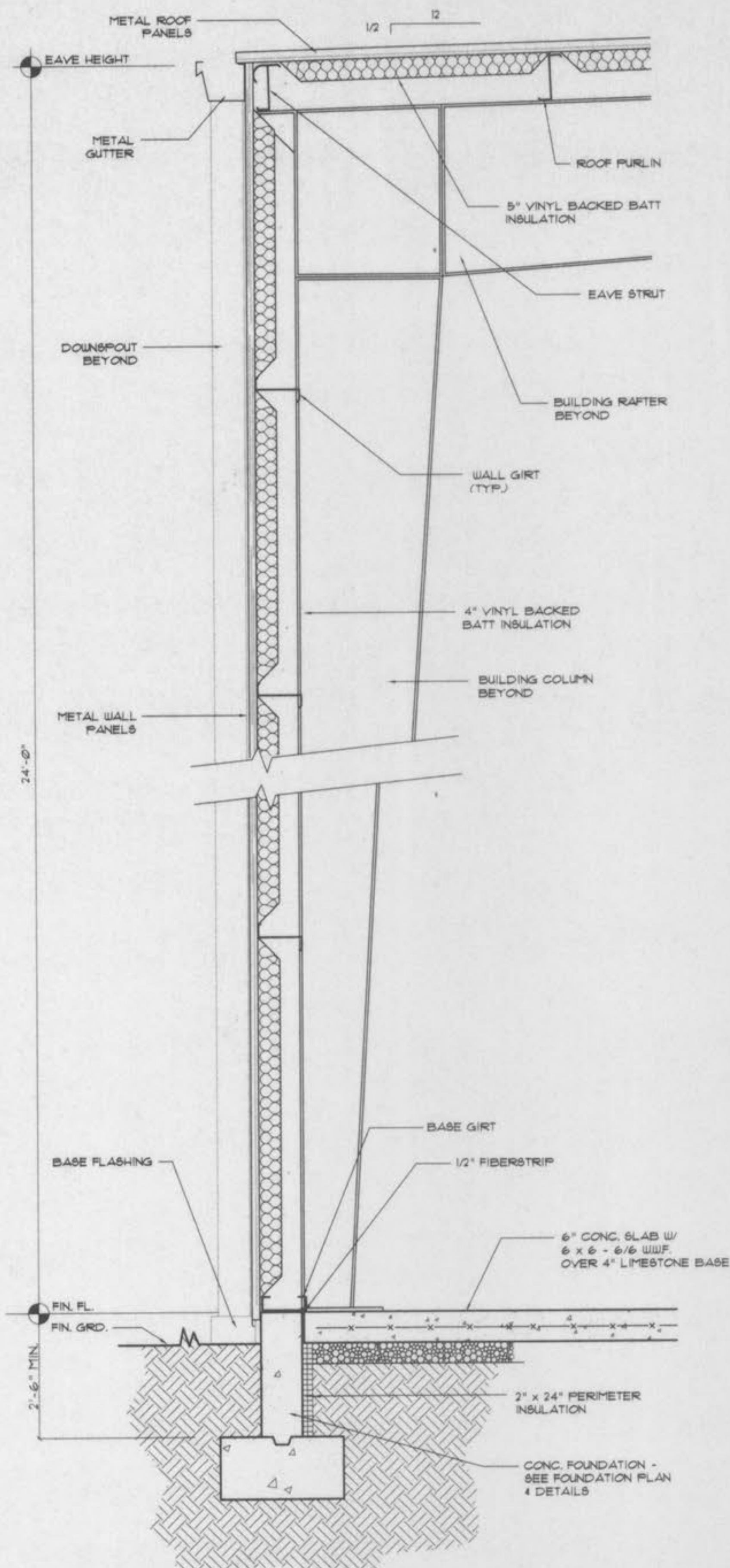
2 24 SECTION THRU SIDEWALL SCALE: 3/4" = 1'-0"
