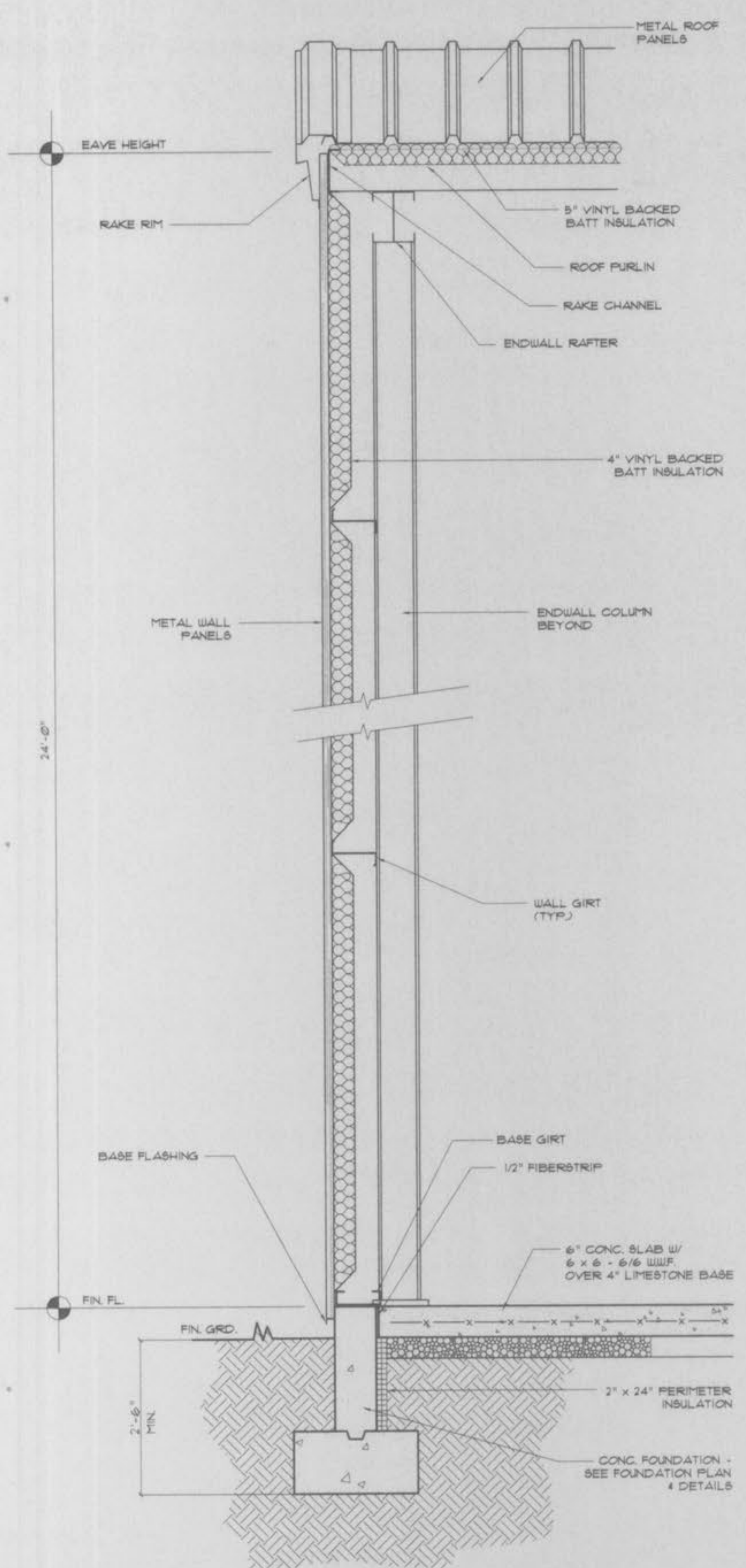
3 24 SECTION THRU WEST ENDWALL SCALE: 3/4" = 1'-0"
