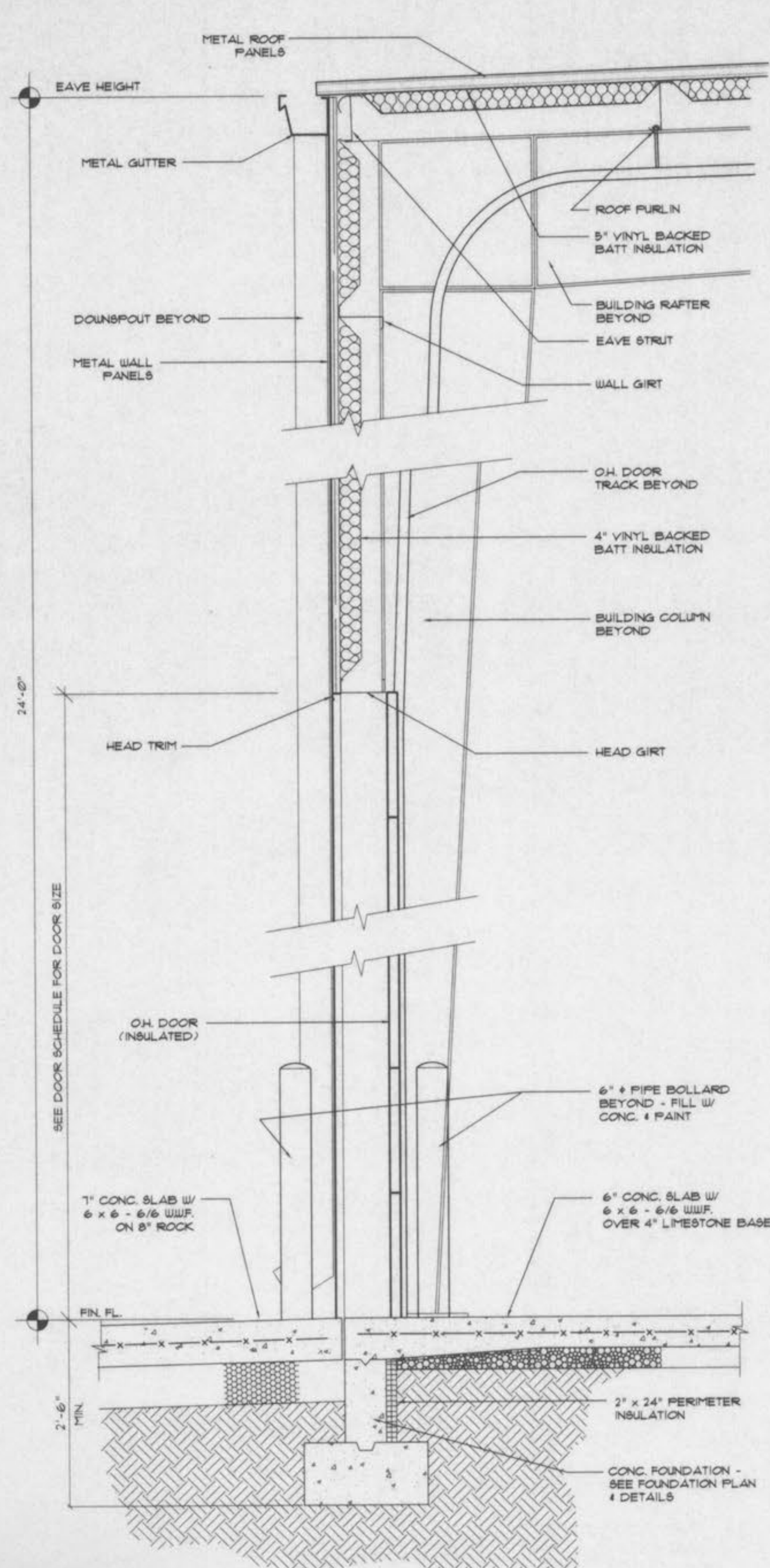
1 24 SECTION THRU SOUTH WALL @ DRIVE-THRU DOOR SCALE: 3/4" = 1'-0"
