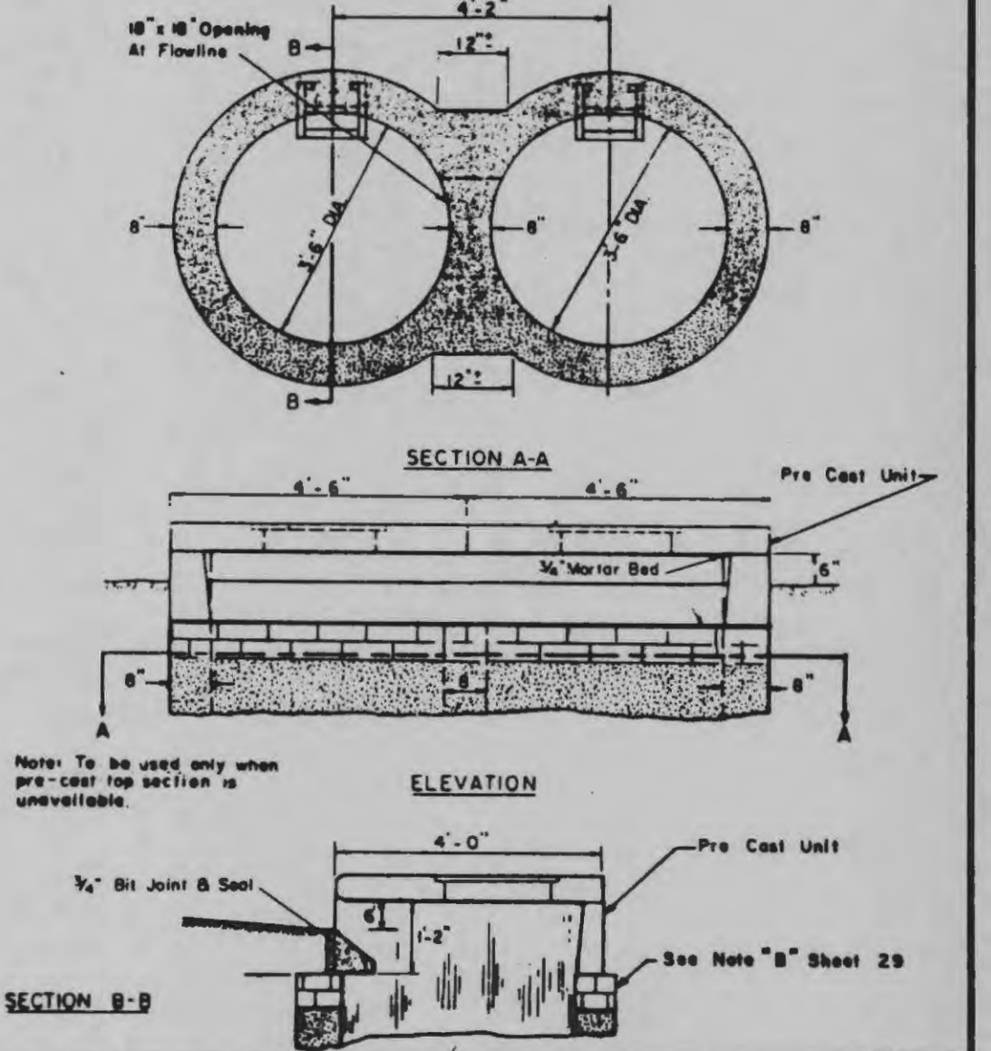
DETAIL 24 CONCRETE DOUBLE STREET INLET W/PRE CAST TOP UNIT
