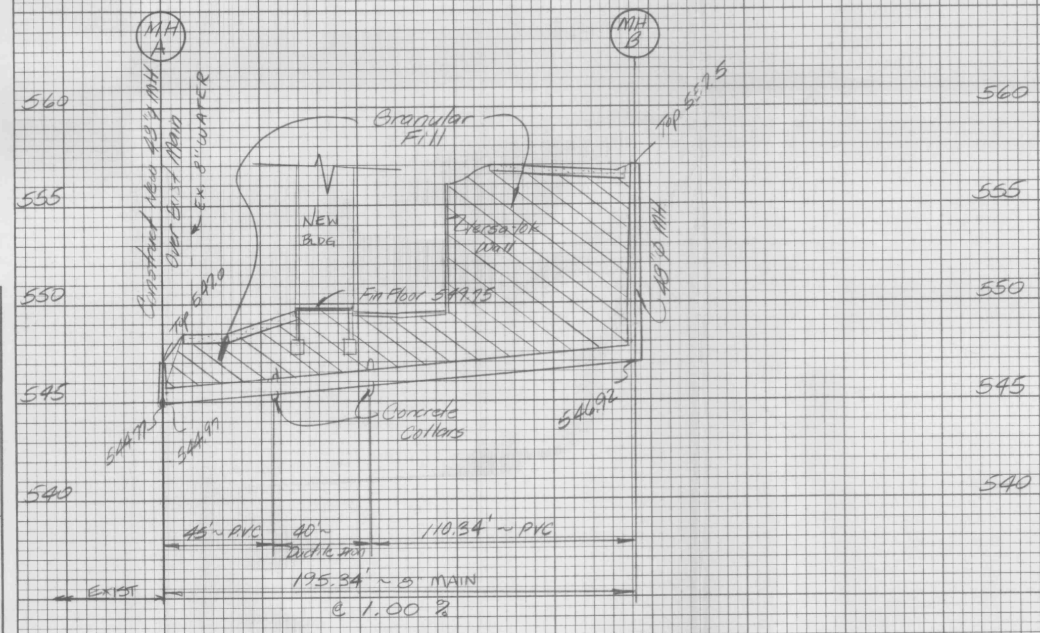
NEW SANITARY SEWER PROFILE SCALE: 1"=40' HORIZ. 1"=5' VERT.
