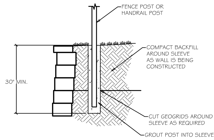
FENCE DETAIL NOT TO SCALE
