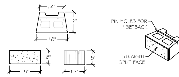
VERSA-LOK SQUARE FOOT UNIT NOT TO SCALE
