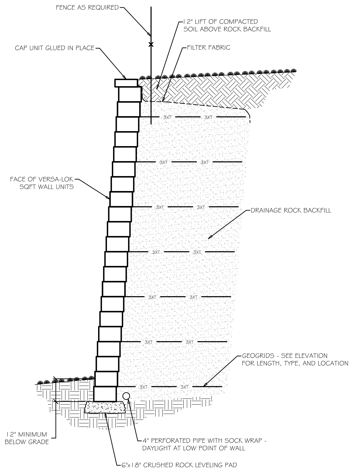
TYPICAL SECTION NOT TO SCALE
