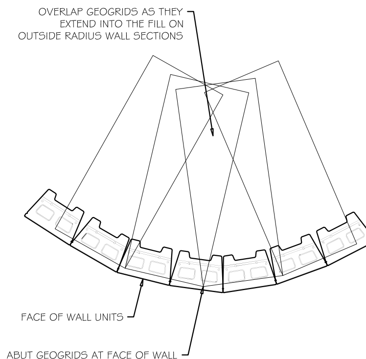
OUTSIDE RADIUS DETAIL NOT TO SCALE
