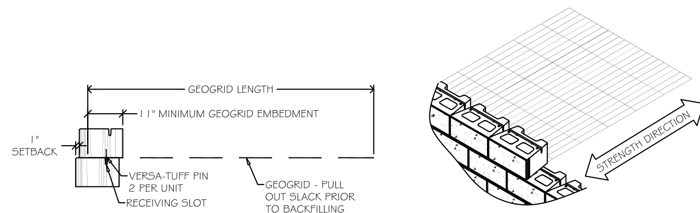
CONNECTION DETAIL NOT TO SCALE
