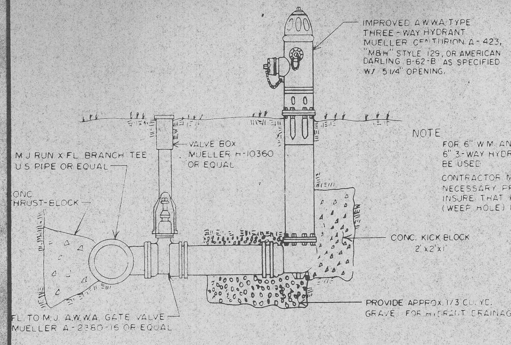
FIRE HYDRANT INSTALLATION DETAIL NO SCALE
