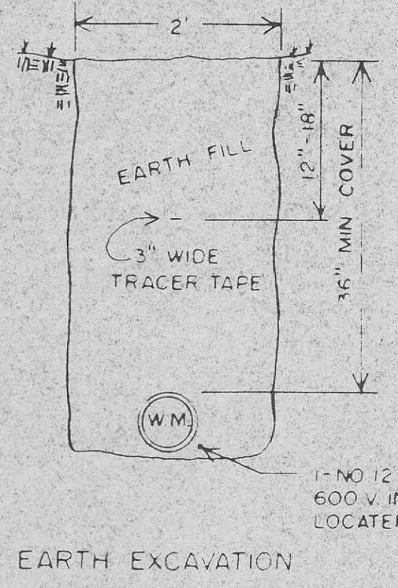
TYPICAL WATER MAIN TRENCHING NO SCALE
