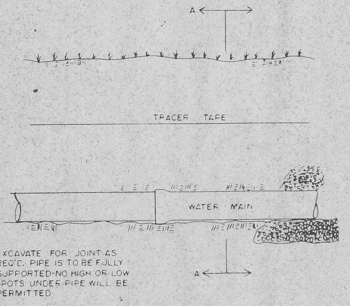
TYPICAL WATER MAIN TRENCHING NO SCALE
