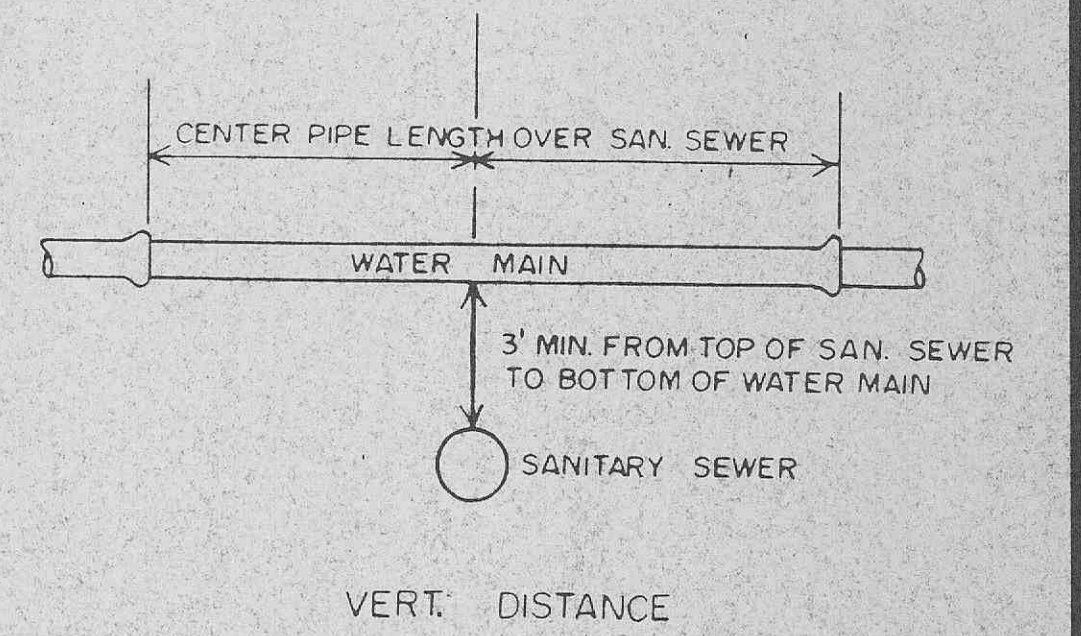
TYPICAL WATER & SEWER SEPARATION NO SCALE
