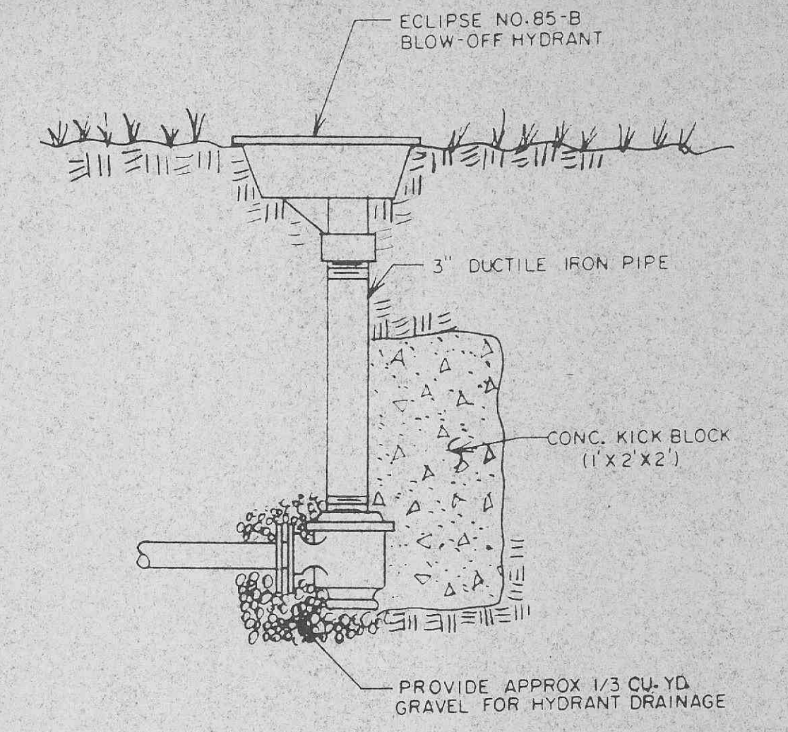
BLOW-OFF HYDRANT NO SCALE
