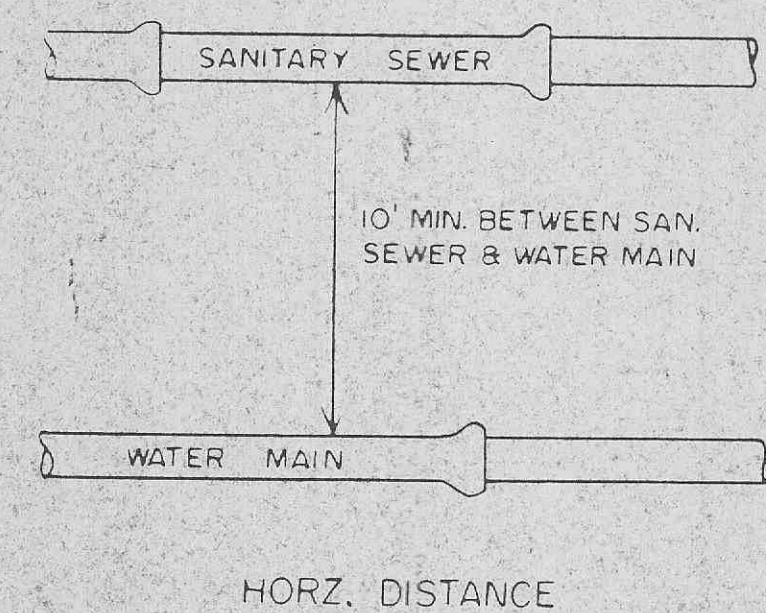
TYPICAL WATER & SEWER SEPARATION NO SCALE
