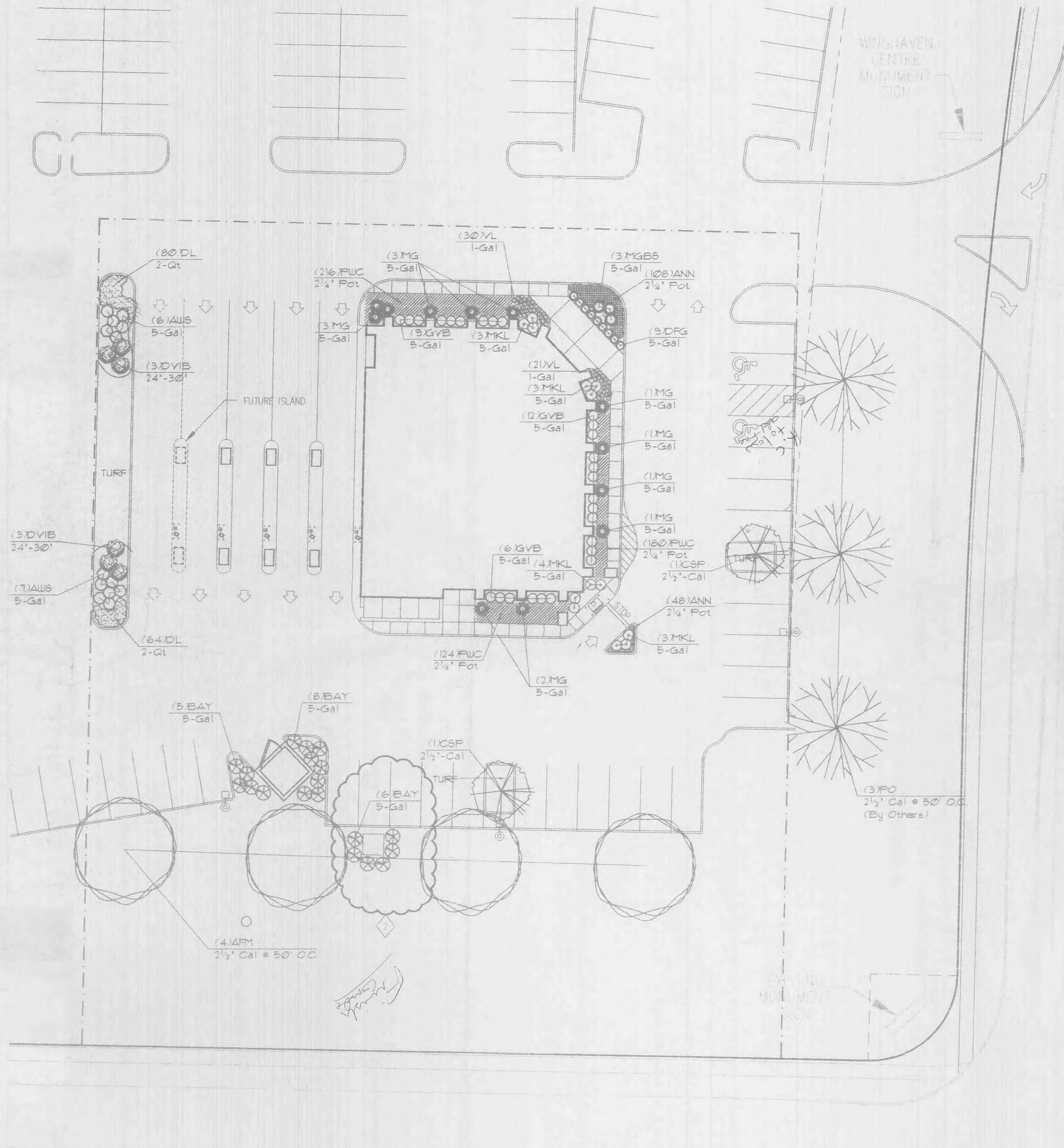
LANDSCAPE PLAN SCALE: 1" = 20'-0"
