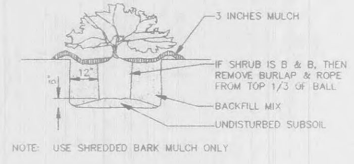
3 SHRUB PLANTING DETAIL NOT TO SCALE
