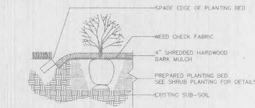
2 SPADE-CUT EDGE DETAIL NOT TO SCALE
