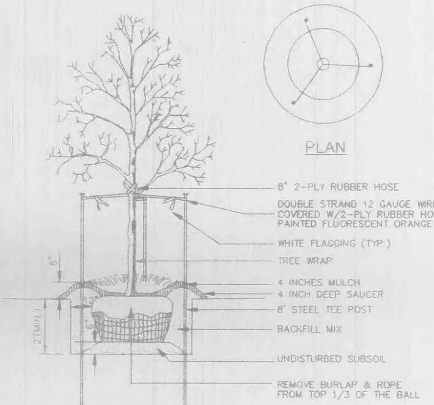
5 DECIDUOUS TREE PLANTING DETAIL NOT TO SCALE
