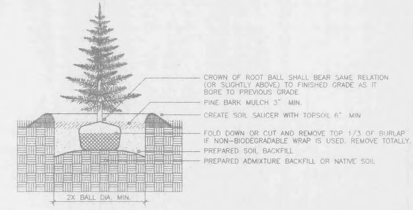
6 EVERGREEN TREE PLANTING DETAIL NOT TO SCALE
