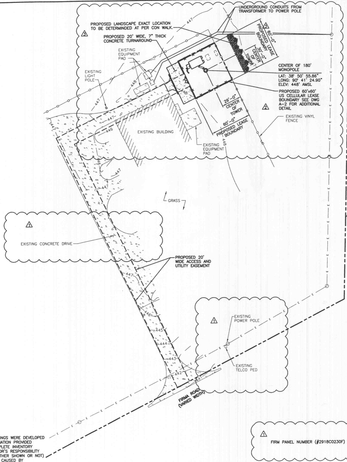
OVERALL SITE PLAN
