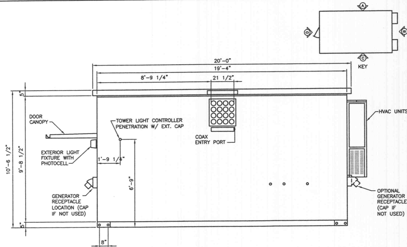
CELLXION EQUIPMENT SHELTER ELEVATION - "A"
