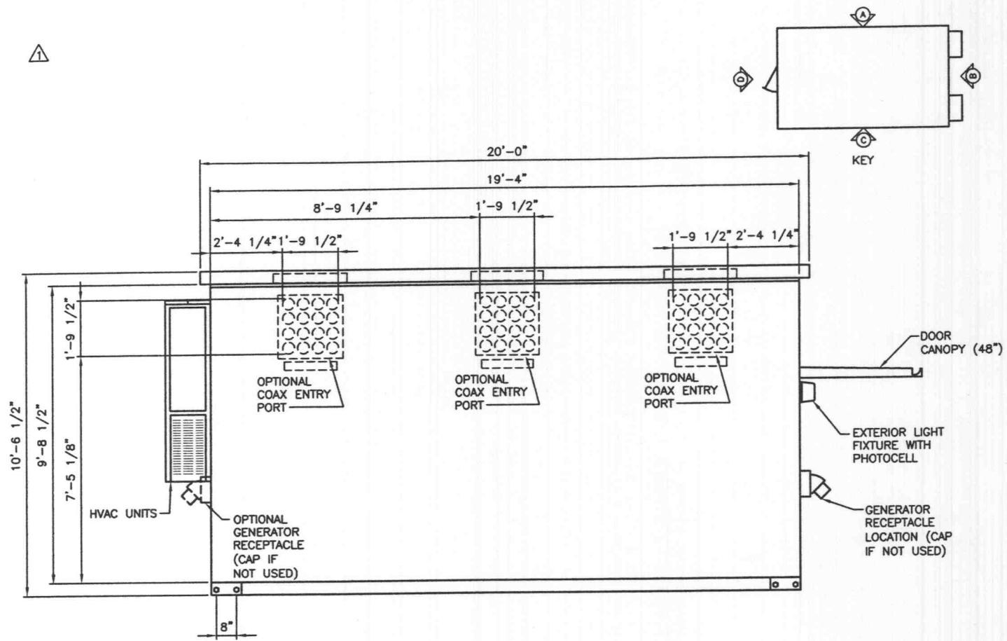
CELLXION EQUIPMENT SHELTER ELEVATION - "A"
