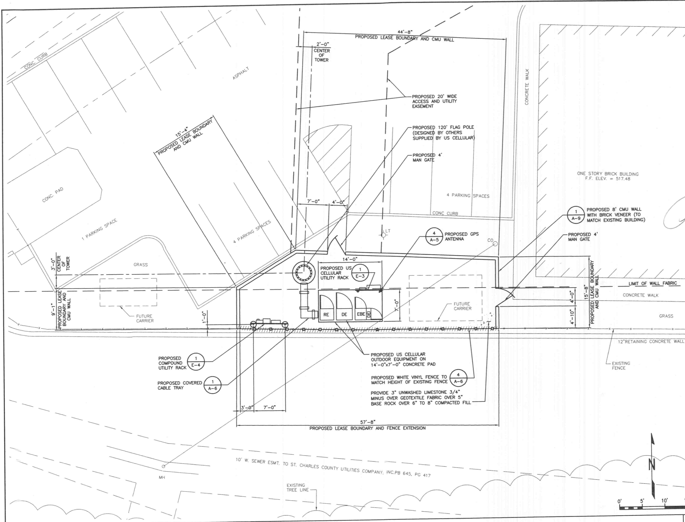
ENLARGED SITE PLAN
