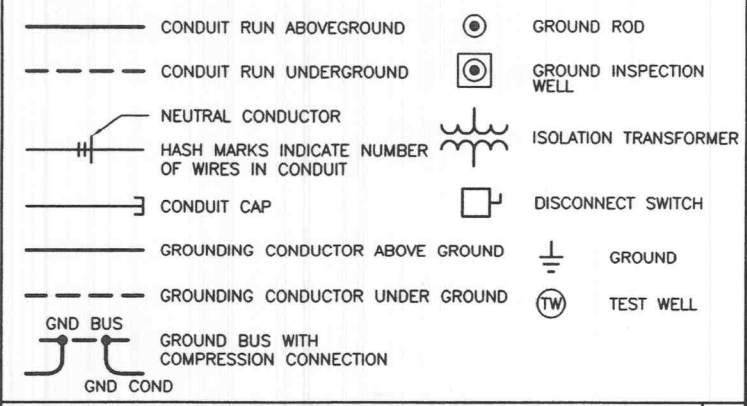
1 ELECTRICAL SYMBOLS
