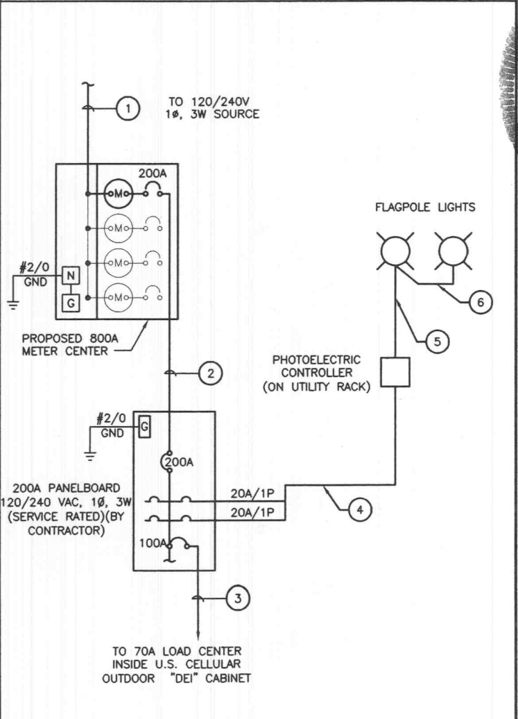
3 ONE-LINE DIAGRAM
