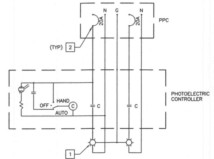
6 PHOTOELECTRIC CONTROL SCHEMATIC 4
