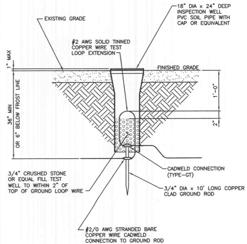
INSPECTION WELL
