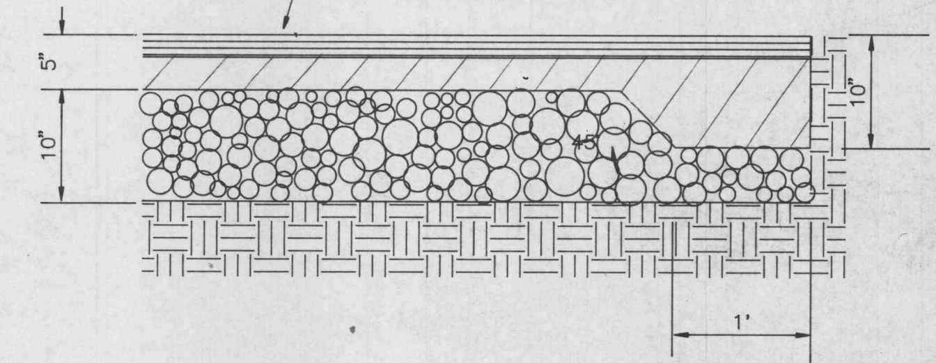
TURNED DOWN EDGE AT HEAVY DUTY ASPHALT PAVEMENT NO SCALE
