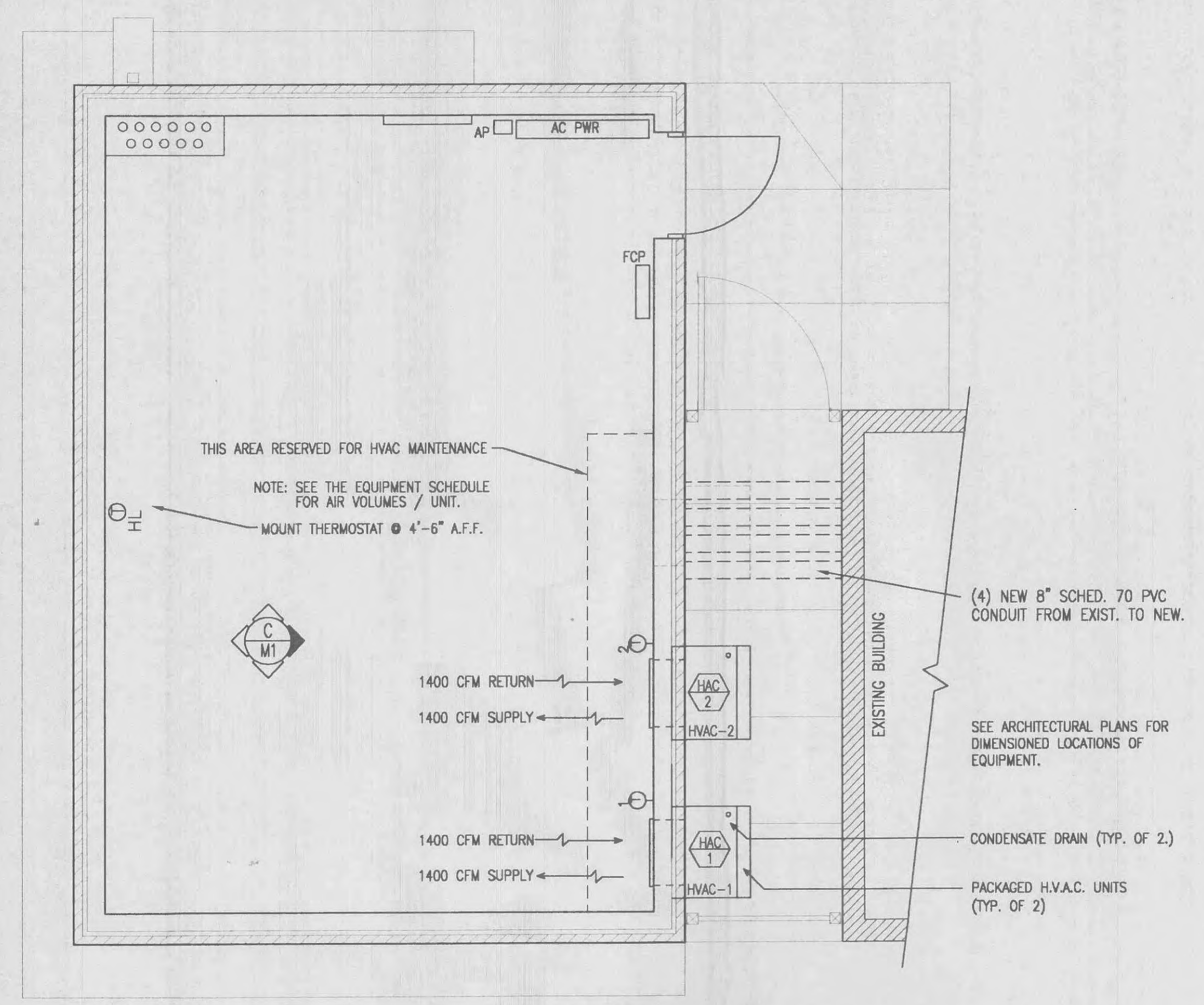
MECHANICAL PLAN 1/4" = 1'-0"
