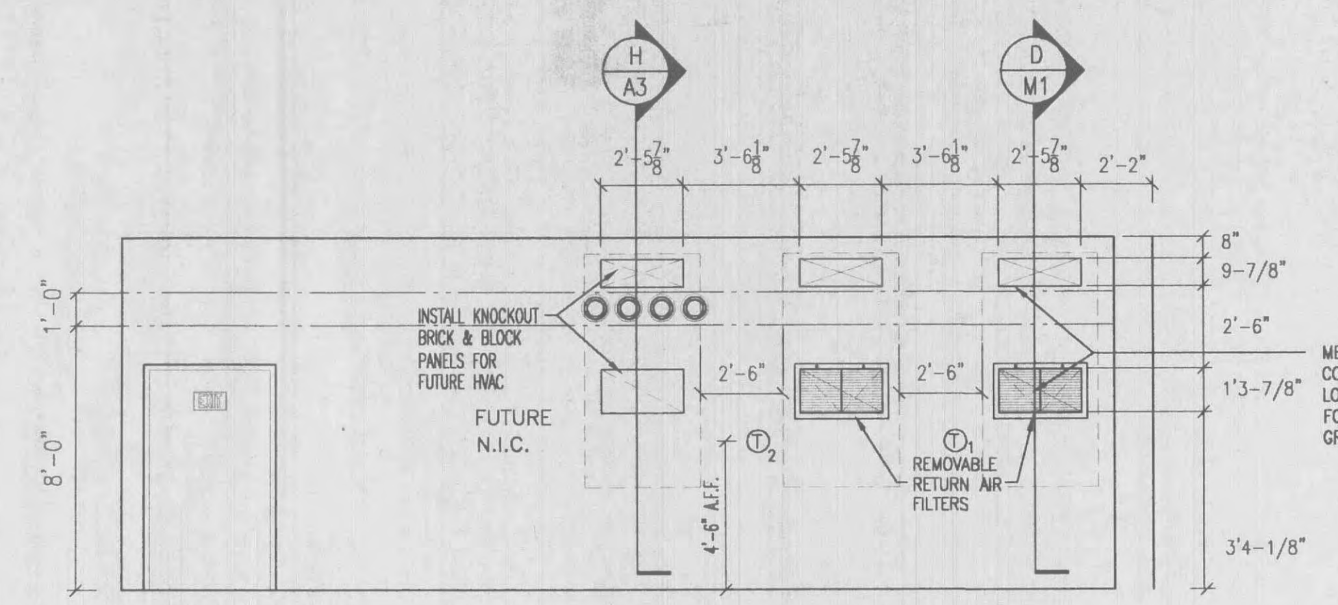
INTERIOR ELEVATION 1/4" = 1'-0"
