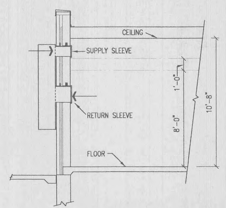
SECTION 1/4" = 1'-0"
