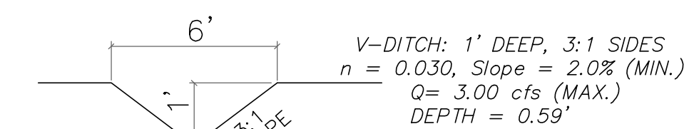
REAR YARD SWALE (TYP.) NOTE: DITCH TO BE EITHER SODDED OR SEEDED & MULCHED.
