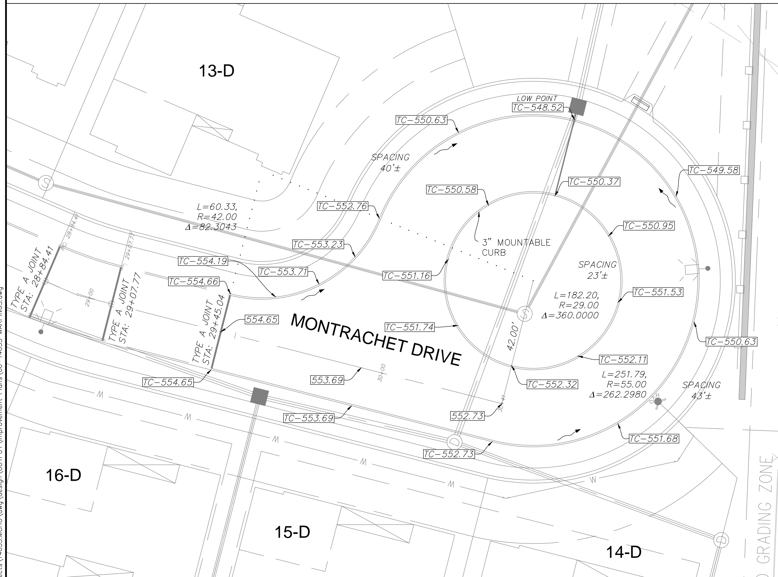
MONTRACHET DRIVE CUL-DE-SAC SCALE 1"= 20'
