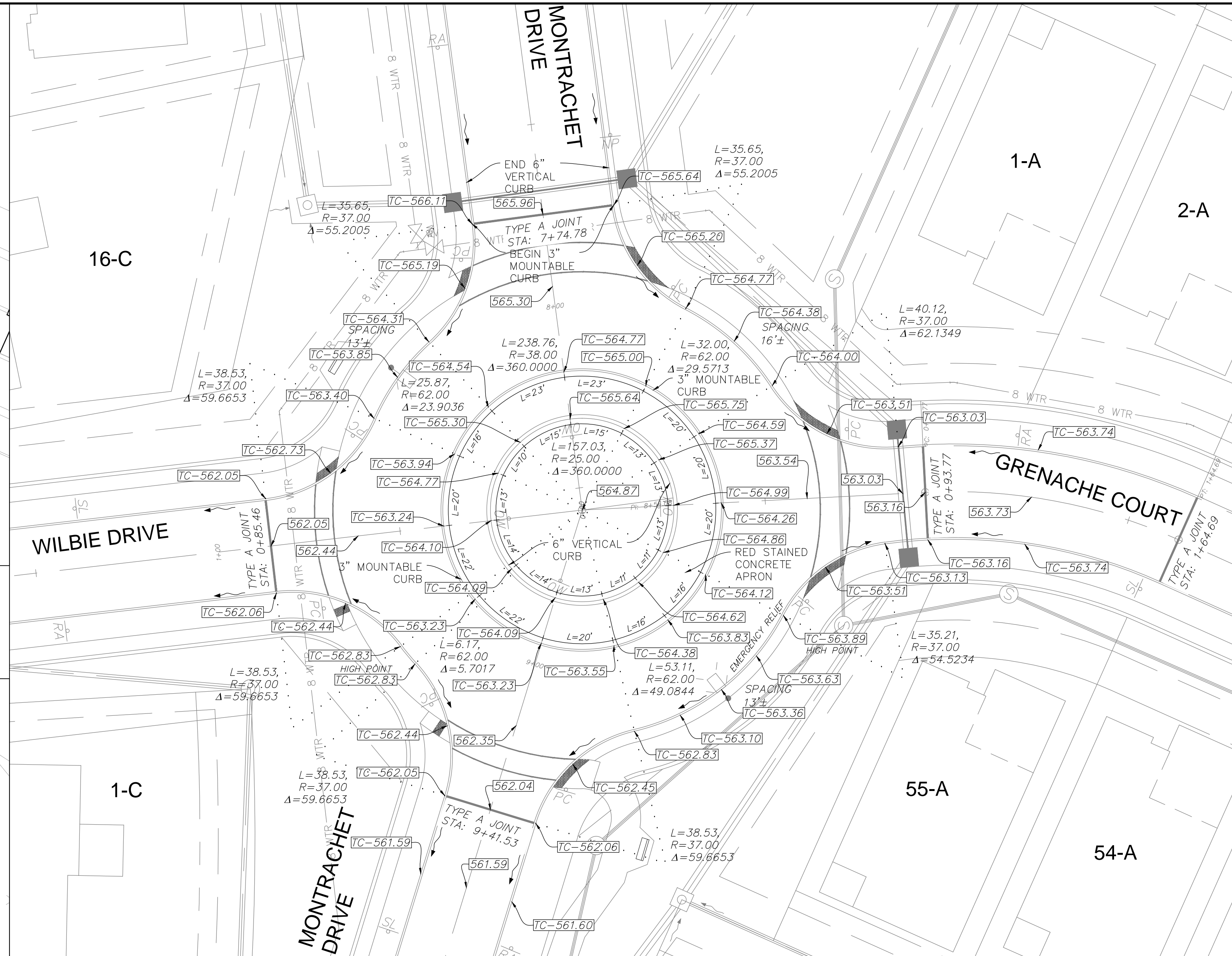
ROUND-A-BOUT SCALE 1"= 20'
