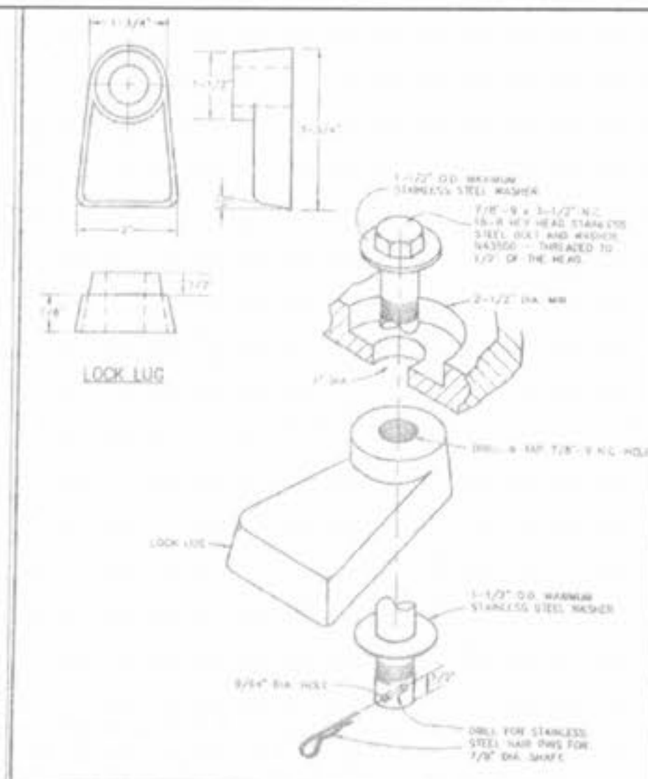
LOCKING DEVICE FOR TYPE "N" LOCK TYPE MANHOLE COVER METROPOLITAN ST. LOUIS SEWER DISTRICT Standard Details of Sewer Construction D. R. H. / S. A. M. Ch. J. C. K. 2000 SHEET 56
