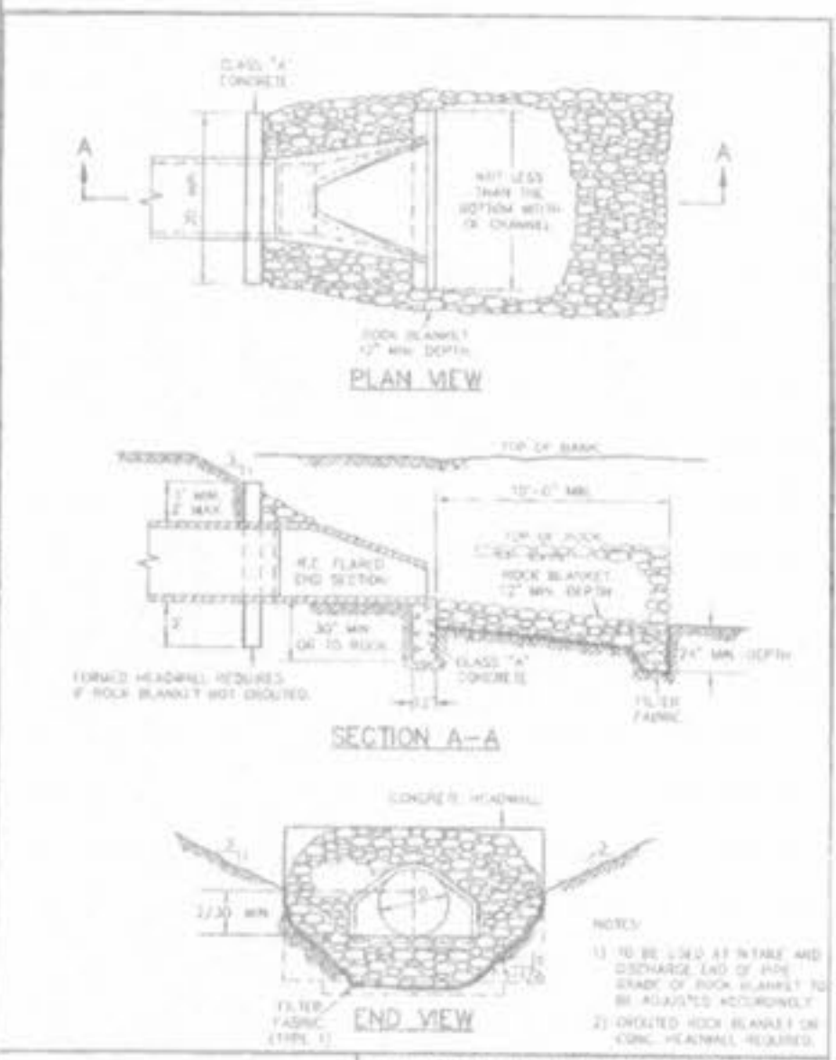
FLARED END SECTION METROPOLITAN ST. LOUIS SEWER DISTRICT Standard Details of Sewer Construction D. R. H. / S. A. M. Ch. J. C. K. 2000 SHEET 61
