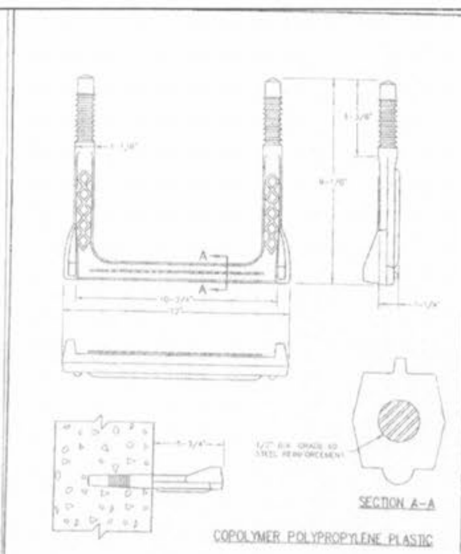
MANHOLE STEP FOR PRECAST & CAST-IN-PLACE MANHOLE METROPOLITAN ST. LOUIS SEWER DISTRICT Standard Details of Sewer Construction D. R. H. / S. A. M. Ch. J. C. K. 2000 SHEET 58
