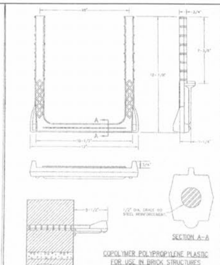
PST-B MANHOLE STEP INTO JOINT METROPOLITAN ST. LOUIS SEWER DISTRICT Standard Details of Sewer Construction D. R. H. / S. A. M. Ch. J. C. K. 2000 SHEET 57
